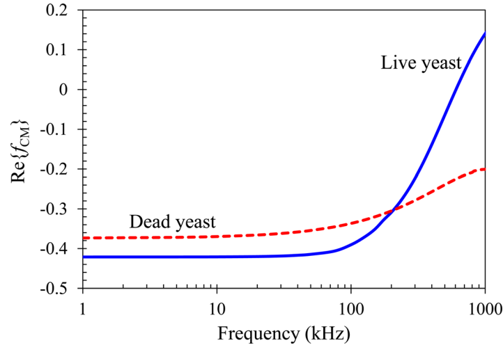
FIG. 3. Comparison of the model predicted CM factors of live (solid line) and dead (dashed line) yeast cells suspended in 1 mM phosphate buffer as a function of the electric field frequency. The dashed-dotted line divides the diagram to positive DEP (top half, \text{Re}\{f_{CM}\} > 0 ) and negative DEP (bottom half, \text{Re}\{f_{CM}\} < 0 ) regions.
