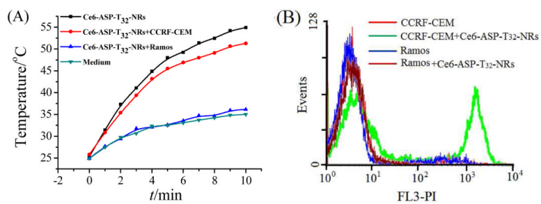
Figure 7. (A) Temperature-time curves of Ce6-labeled ASP-T 32 -NR complex and (B) photothermal therapy (PTT) results with laser irradiation. sgc8-NRs, 0.2 nM; cells, 200 k/sample; probes, 200 nM; laser wavelength, 812 nm.
