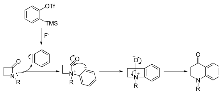
Scheme 1. Originally anticipated reaction of a \beta -lactam with an aryne
