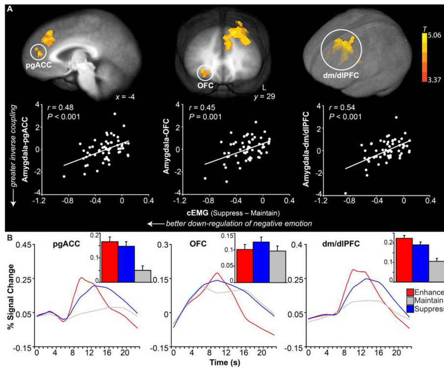
Figure 4. Amygdala-PFC connectivity supporting down-regulatory success. Individual differences in down-regulatory ability predicted amygdala-PFC functional connectivity 1.3 years later. (A) Top panel depicts PFC clusters showing functional connectivity with amygdala during suppress versus maintain as predicted by cEMG difference scores (Suppress – Maintain). Bottom panel illustrates scatterplots between amygdala-PFC connectivity (y-axis; standardized mean beta) for each identified region above, and cEMG regulation success (x-axis; \mu V^2/Hz ) obtained 1.3 years earlier. Individuals who were more successful at down-regulating negative emotion (more negative cEMG scores) exhibited greater inverse amygdala-PFC coupling during down-regulation of negative emotion (more negative betas), while individuals who were worse at regulation showed more positive coupling. (B) BOLD signal changes by regulatory instruction over time in the PFC regions implicated in this functional connectivity analysis. Inset figures represent the main effects of regulation. Error bars indicate the SEM_{\text{difference}} .
