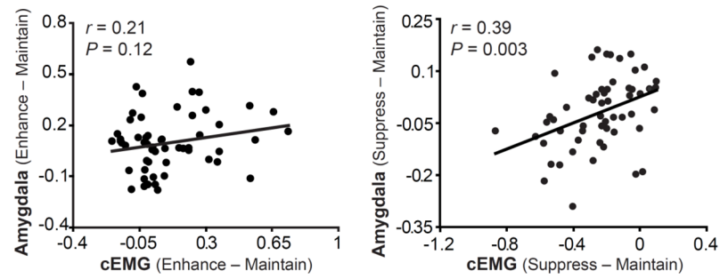
Figure 3. Stability of emotion regulatory success across sessions. The ability to down-regulate negative emotion assessed using cEMG ( \mu V^2/Hz ) and amygdala activity (% signal change) were moderately correlated over the 1.3-year interval. However, the ability to up-regulate negative emotion was not significantly correlated.
