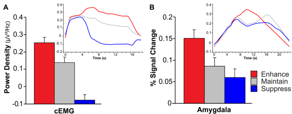
Figure 2. Effects of emotion regulation on (A) cEMG activity (session 1) and (B) amygdala BOLD signal (session 2). For both sessions, participants regulated their responses to negative pictures according to instructions. Error bars indicate the SEM_{\text{difference}} . Inset figures illustrate the time series of cEMG and amygdala activity.
