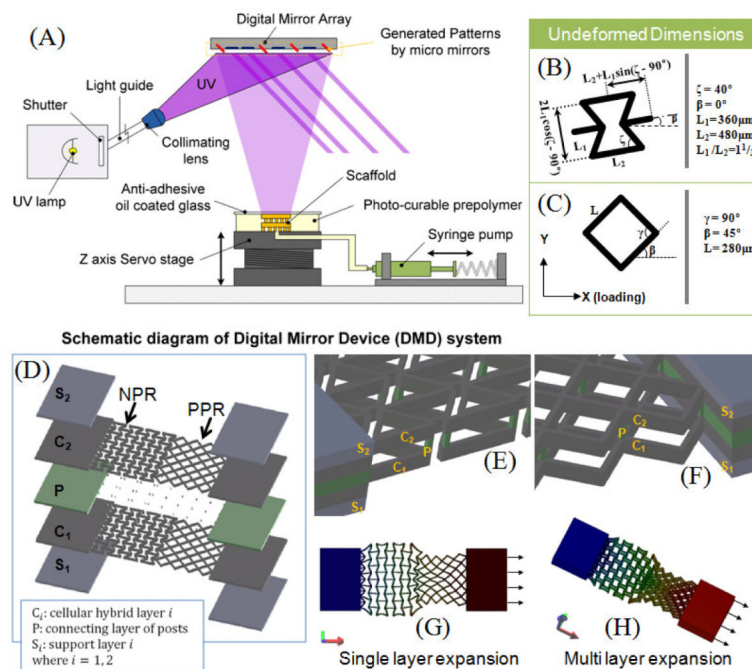
Figure 1. (A) Schematic of the digital micromirror device micro-stereolithography system (DMD-SL) used for fabricating single- and multi-layer scaffolds having NPR-PPR regions. (B,C) Unit-cell geometry and relevant dimensional parameters having the negative Poisson ratio (NPR) [44, 45, 49], and positive Poisson's ratio (PPR) [43]. (D) Schematic of the two-layer scaffold assembled by stacking single-layer scaffolds with a connecting layer of vertical posts (P); (E,F) magnified views of the double-layer stacks. (G,H) stress-strain simulations of single and two-layer PEG scaffolds composed of unit-cells (The walls of the unit-cells (denoted as struts) are approximately 40 \mu\text{m} wide and 100 \mu\text{m} deep).
