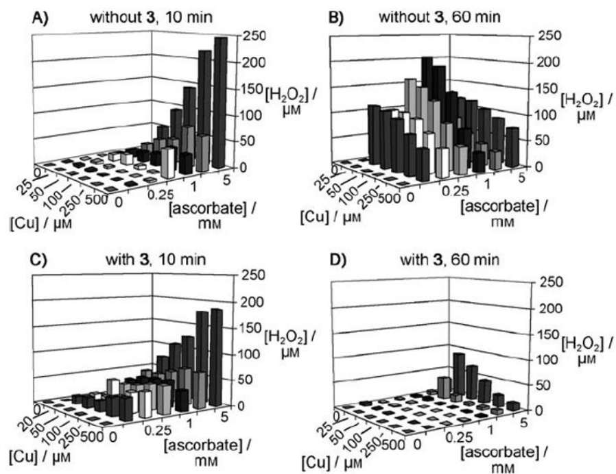
Figure 3. Hydrogen peroxide formation in the presence of various concentrations of CuSO_4 (0–500 \mu M ) and sodium ascorbate (0–5 mM), monitored by fluorescence of amplex red ( \lambda_{ex}=570 nm, \lambda_{em}=590 nm) in the presence of horseradish peroxidase at 10 and 60 min after addition of ascorbate: A,B) In the absence of ligand 3 ; C,D) in the presence of 5 equivalents of ligand 3 with respect to Cu.
