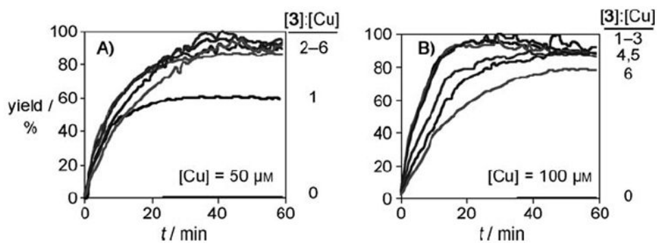
Figure 1. Conversion–time profiles as a function of ligand/Cu ratio. Conditions: propargyl alcohol (100 μM), 1 (50 μM), CuSO 4 , and ligand 3 (indicated concentrations), 0.1M potassium phosphate buffer (pH 7.0)/DMSO 95:5, sodium ascorbate (5.0 mM), room temperature.
