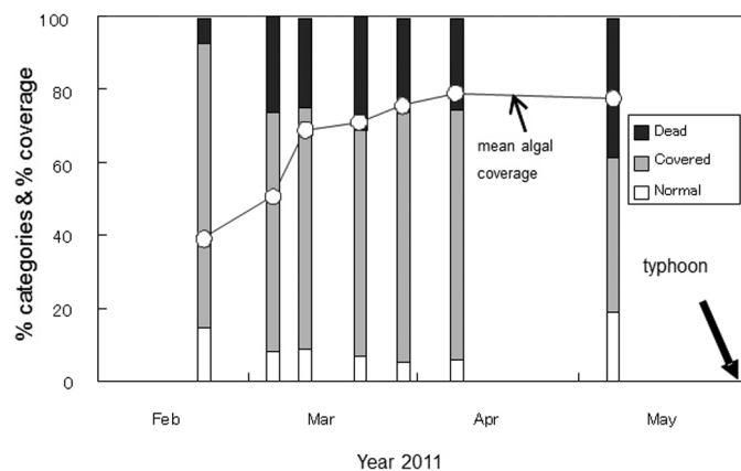
Figure 4 | Changes in algal covers as a mean algal coverage (%) in whole colonies, and as three categories (% dead, % covered with diatoms, and % normal colonies). Periodical census started on Feb 20 th and finished on 7 th May before a strong typhoon on 28 th May 8 in 2011.
