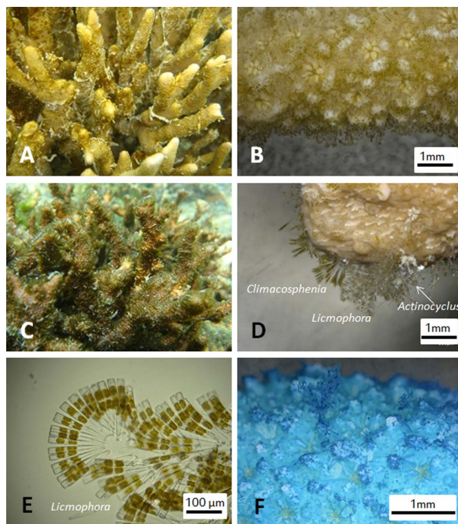
Figure 3 | Diatoms covering Montipora coral. A, Attached diatoms are visible as brown patches, and the coral secretes mucus strands against them. B, A coral branch covered by numerous diatoms ( Licmophora ). C, Advanced stage showing fluffy branches. D, Attached diatoms around the growing chip. E, Licmophora flabellata showing fan-like colony and branched mucilage stalks. F, Coral surface stained with Alcian blue, most diatoms are detached leaving pads on the protuberant bared skeleton.
