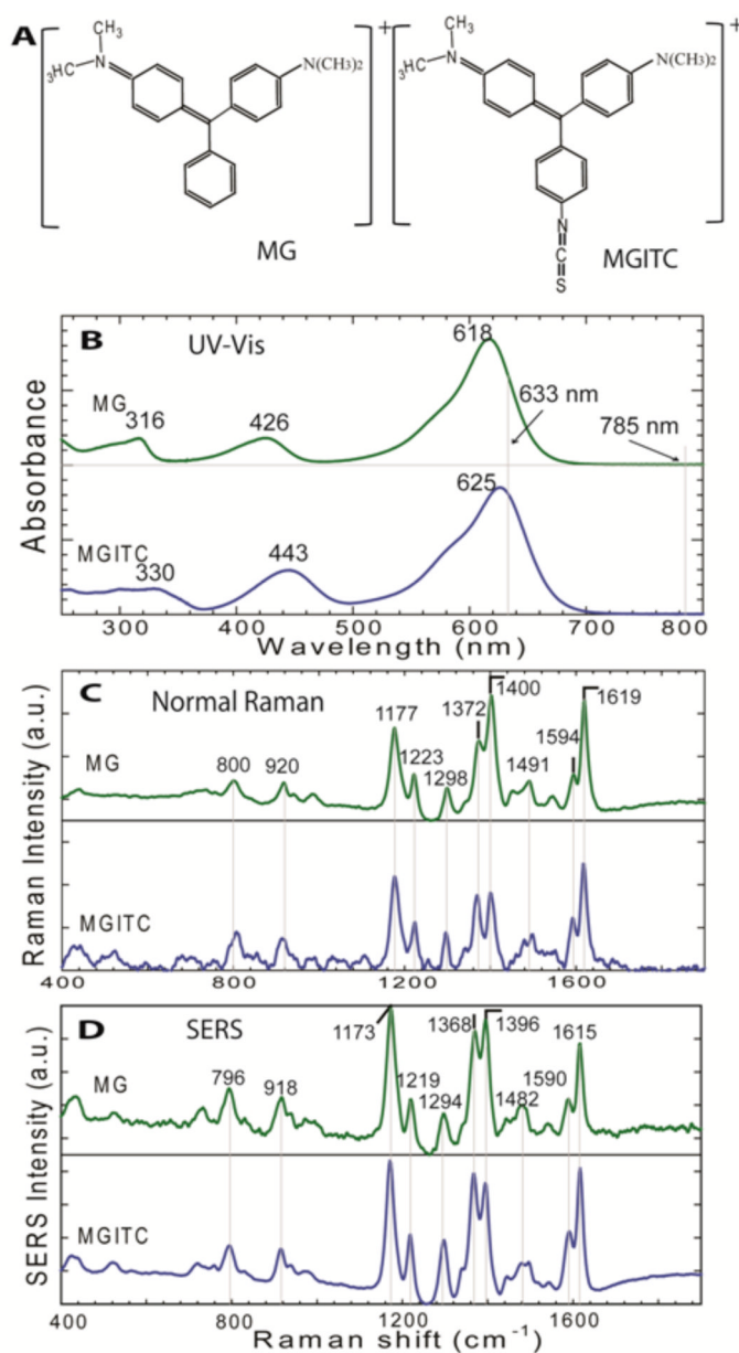
Figure 1. Malachite green (MG) and its isothiocyanate derivative (MGITC), two organic chromophores that have very different functional groups for attaching to gold surfaces, but nearly identical spectroscopic properties. (A) Schematic chemical structures of MG and MGITC in their delocalized electronic forms (with delocalized \pi -electrons); (B) Comparison of UV-Vis absorption spectra between MG and MGITC; (C) normal Raman spectra and (D) SERS spectra of MG and MGITC. The normal Raman spectra were obtained from MG (2.5 mM) and MGITC (1 mM) in water solution with 2-sec integration time, and were plotted on the same intensity scale. The SERS spectra were obtained from a colloidal gold solution (60-nm particle diameter, 14-pM concentration) mixed with 2.3 \mu\text{M} MG or 0.2 \mu\text{M} MGITC at room temperature, 1-sec integration time. All Raman measurements were acquired by using 785-nm laser excitation, 40-mW laser power. Note that the SERS signal
