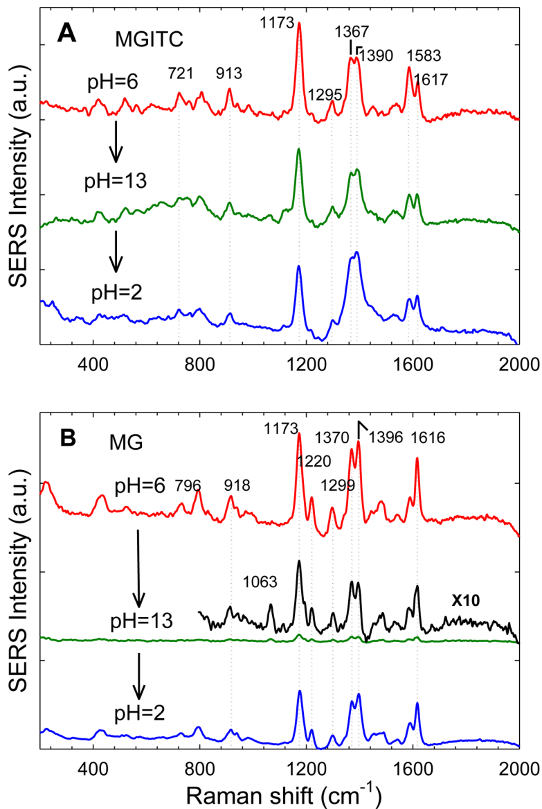
Figure 3. SERS spectra of MGITC (A) and MG (B) obtained with 785 nm laser excitation as a function of pH. As the pH was changed sequentially from 6 to 13 and then to 2, the isothiocyanate dye was found irreversibly stabilized or “locked” in its \pi -conjugated structure whereas the adsorbed malachite green was still sensitive to pH and could be switched between its localized and delocalized forms. Laser power = 40 mW; integration time = 20 s.
