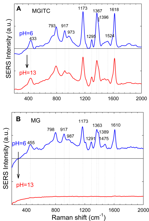
Figure 4. SERRS spectra of MGITC (A) and MG (B) obtained with 633 nm laser excitation at acidic or basic pHs (pH = 6 or 13). Note that the electronic structure of adsorbed MGITC is locked in its delocalized form and is no longer sensitive to pH, whereas the structure of adsorbed MG is still sensitive to pH and can be switched between its localized and delocalized forms. The laser power was 3 mW, and the integration time was 1 sec.
