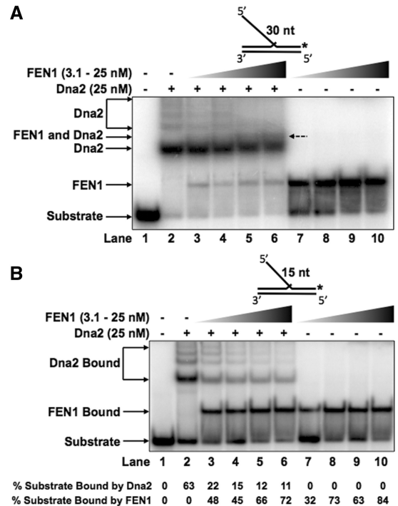
Figure 4. FEN1 preferentially displaces Dna2 from intermediate length double-flap structures. Dna2 (25 nM) was pre-incubated with the experimental substrate prior to the addition of increasing concentrations of FEN1 (3.1, 6.25, 12.5 or 25 nM in lanes 3-6). Lane 1 shows the substrate alone, lane 2 shows Dna2 bound without FEN1 and lanes 7-10 show FEN1 alone bound to the substrate at the same concentrations as in 3-6. (A) shows Dna2 and FEN1 binding competition for the 30 nt double-flap substrate (U2:T3:D2.30). (B) shows Dna2 and FEN1 binding competition for the 15 nt double-flap substrate (U2:T3:D2.15). In (A) and (B) the position of the substrate alone, Dna2-substrate complex and FEN1-substrate complex are indicated to the left of the figure. In (A), the FEN1-Dna2-substrate complex is indicated to the left of the figure and to the right of lane 6 with a dashed arrow. In (B), the quantitation of the percent substrate bound by hDna2 or hFEN1 is shown below the figure.
