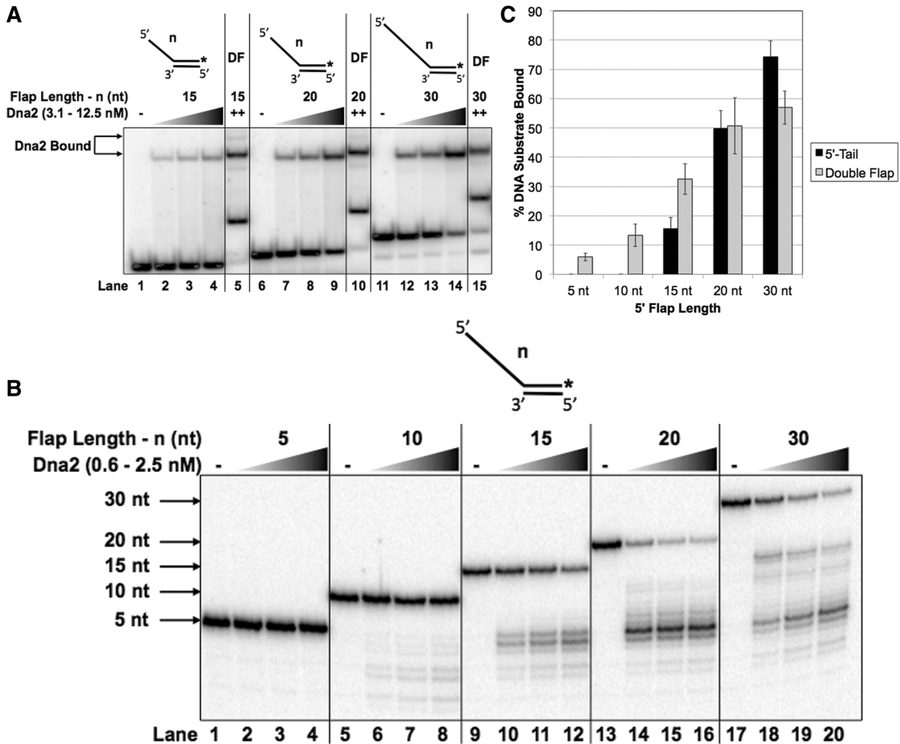
Figure 2. Dna2 demonstrates reduced binding for intermediate 5'-tail structures relative to double flaps. (A) shows Dna2 binding to the 5'-tail substrates having a 5' flap of 15 nt (T2:D1.15), 20 nt (T2:D1.20) or 30 nt (T2:D1.30). The double-flap substrates have a 5' flap of 15 nt (U1:T1:D1.15), 20 nt (U1:T1:D1.20) or 30 nt (U1:T1:D1.30). Binding was measured by EMSA using increasing Dna2 concentrations (3.1, 6.25 or 12.5 nM). (B) shows Dna2 cleavage of 5'-tail substrates having a 5' flap of 5 nt (T2:D1.5), 10 nt (T2:D1.10), 15 nt (T2:D1.15), 20 nt (T2:D1.20) or 30 nt (T2:D1.30). Cleavage was measured by denaturing gel electrophoresis using increasing concentrations of Dna2 (0.6, 1.25 or 2.5 nM). (C) shows the graphical quantitation of 12.5 nM Dna2 from (A). In (A), the position of the Dna2-substrate complex is indicated to the left of the figure. '++' represents the maximum concentration of Dna2 used. 'DF' represents the lane containing the double-flap structure. In (B), the position of the radiolabeled oligonucleotide is indicated to the left of the figure. The experimental 5'-tail substrate configuration is shown above each figure where 'n' represents the length of the 5' flap.
