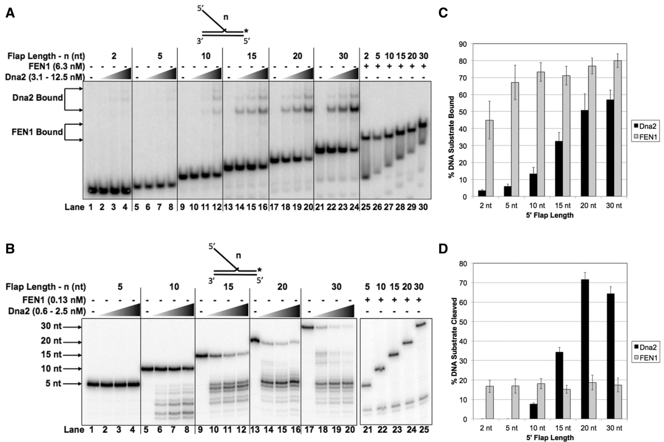
Figure 1. Dna2 binding correlates to cleavage on Okazaki fragment double-flap structures. Dna2 and FEN1 binding and nuclease activity of double-flap substrates having a 5' flap of 2 nt (U1:T1:D1.2), 5 nt (U1:T1:D1.5), 10 nt (U1:T1:D1.10), 15 nt (U1:T1:D1.15), 20 nt (U1:T1:D1.20) or 30 nt (U1:T1:D1.30) were measured by EMSA and denaturing gel electrophoresis, respectively, as described in the 'Material and Methods' section. (A) shows Dna2 (3.1, 6.25 and 12.5 nM) and FEN1 (6.25 nM) binding to the double-flap substrates. (B) shows Dna2 (0.6, 1.25 and 2.5 nM) and FEN1 (0.13 nM) cleavage of the double-flap substrates. (C) shows the graphical quantitation of 12.5 nM Dna2 and 6.3 nM FEN1 from (A) and (D) shows the quantitation of 0.63 nM Dna2 and 0.13 nM FEN1 from (B). In (A), the position of the Dna2-substrate complex and FEN1-substrate complex are indicated to the left of the figure. In (B), the position of the radiolabeled oligonucleotide is indicated to the left of the figure. The experimental substrate configuration is shown above each figure where 'n' represents the length of the 5' flap.
