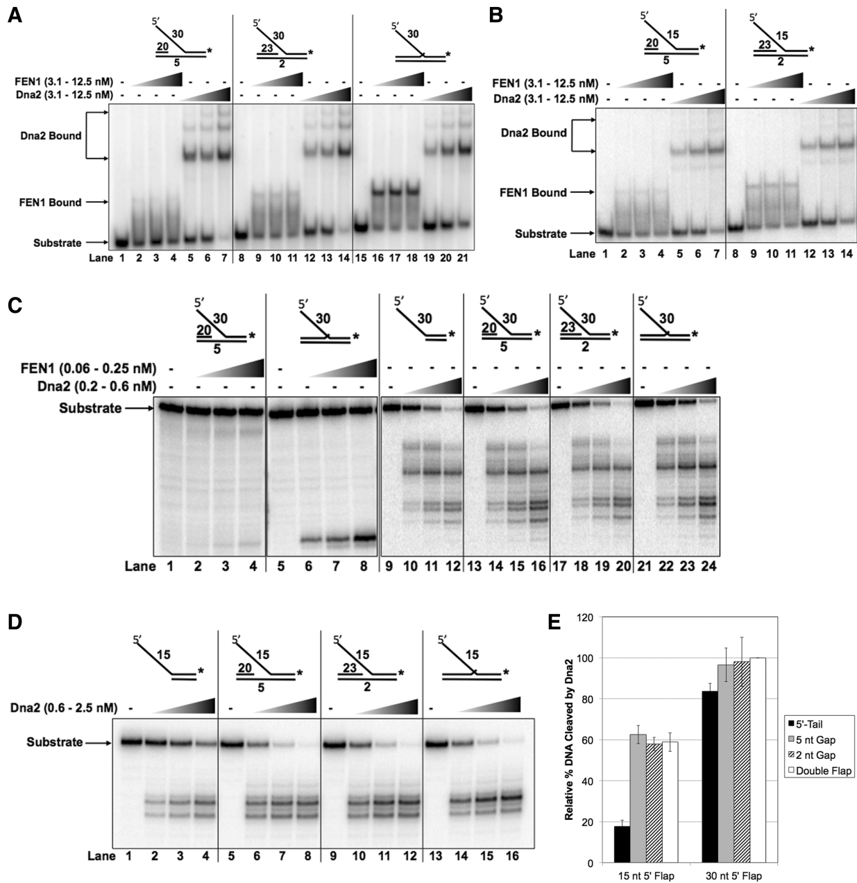
Figure 3. Dna2 binding is improved by the upstream region for short flap structures while stable FEN1 binding requires the full upstream region. (A) shows Dna2 or FEN1 binding to the 5 nt gap-flap (U3:T3:D2.30), 2 nt gap-flap (U4:T3:D2.30) and double-flap (U2:T3:D2.30) substrates with 30 nt 5' flaps. (B) shows Dna2 or FEN1 binding to the 5 nt gap-flap (U3:T3:D2.15) and 2 nt gap-flap (U4:T3:D2.15) structures with 15 nt 5' flaps. Binding was measured in (A) and (B) by EMSA using increasing Dna2 and FEN1 concentrations (3.1, 6.25 or 12.5 nM). (C) shows FEN1 cleavage of the 5 nt gap-flap (U3:T3:D2.30) and double-flap (U2:T3:D2.30) structures (lanes 1–8) and Dna2 cleavage of the 5'-tail (T4:D2.30), 5 nt gap-flap (U3:T3:D2.30), 2 nt gap-flap (U4:T3:D2.30) and double-flap (U2:T3:D2.30) structures (lanes 9–24) with 30 nt 5' flaps. (D) shows Dna2 cleavage of the 5'-tail (T4:D2.15), 5 nt gap-flap (U3:T3:D2.15), 2 nt gap-flap (U4:T3:D2.15) and double-flap (U2:T3:D2.15) structures with 15 nt 5' flaps. Nuclease activity was measured by denaturing gel electrophoresis. (E) shows the graphical quantitation of the relative cleavage of 0.63 nM Dna2 from (C) and (D) as defined in the 'Materials and Methods'. In (A) and (B) the position of the substrate alone, Dna2–substrate complex and FEN1–substrate complex are indicated to the left of the figure. In (C) and (D) the position of the radiolabeled oligonucleotide is indicated to the left of the figure. The experimental substrate configurations are shown above figures (A)–(D).
