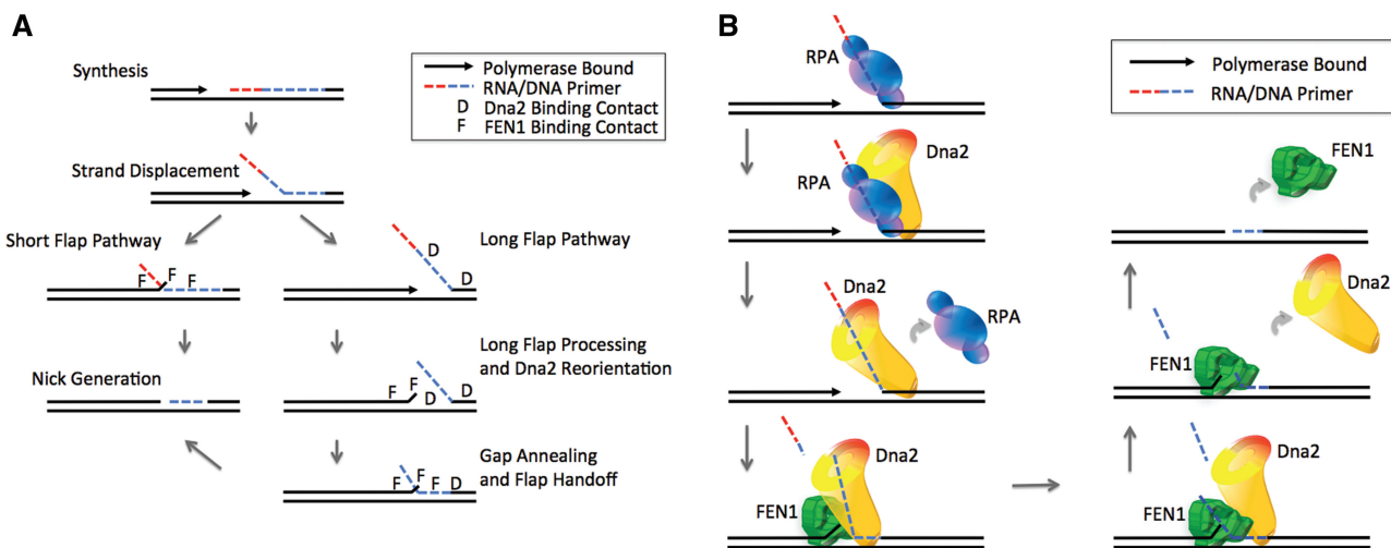
Figure 6. Models of FEN1 and Dna2 Okazaki fragment substrate recognition and processing. (A) hDna2 and hFEN1 substrate recognition model. Pol \delta synthesizes until encountering the downstream Okazaki fragment RNA/DNA primer. Pol \delta then physically separates the two strands of the duplex DNA to form a 5' flap. The active site of the polymerase protects a 5–6 nt single-stranded region on the template creating a structure with a 5'-displaced flap and a single-stranded gap between the upstream and downstream primers, termed a gap-flap. Left arrow: short flap pathway. During short flap processing, the polymerase idles back or dissociates from the synthesis fragment allowing the 5' flap to re-anneal with the template generating a short double-flap structure. hFEN1 binds the double-flap substrate using three contact locations, indicated by 'F', (i) upstream dsDNA, (ii) downstream dsDNA and (iii) the 3' 1 nt flap. Right arrow: long flap pathway. During long flap processing, flaps escape hFEN1 cleavage. hDna2 binds the long gap-flap using two contact locations, indicated by 'D', the downstream dsDNA and the long 5' flap. Dna2 threads the long flap and begins cleaving. The polymerase idles back or dissociates from the synthesis fragment allowing Dna2 to continue to cleave the long flap. hDna2 binding affinity for the 5' flap is reduced and it reorients to bind the upstream DNA. This hDna2 reorientation promotes the re-annealing of the 5' flap with the template, filling the single-stranded gap. The combination of hDna2 upstream DNA binding and the formation of the double flap promote hFEN1 flap base localization. hDna2 releases from the upstream DNA and the 5' flap allowing hFEN1 binding contacts with the upstream dsDNA and the 1 nt 3' flap. The 5' flap transitions to hFEN1 and hFEN1 binds the downstream DNA. hFEN1 is now poised to thread and cleave the substrate and generate a nicked product. (B) Long Flap Pathway Model. As in (A), pol \delta displaces the 5' flap into a 5–6 nt gap-flap structure. Flaps escaping hFEN1 cleavage become long and are bound by hRPA. hDna2 binds the flap displacing hRPA. hDna2 cleaves the long flap as pol \delta idles back or dissociates from the synthesis fragment. hDna2 reorients promoting 5' flap re-annealing with the template, as shown in (A). The double-flap structure formation and hDna2–hFEN1 protein interactions allow hFEN1 to bind the flap base. The reduced hDna2-binding affinity for the shortened 5' flap permits hFEN1 acquisition of the flap for threading. hDna2 stimulates the cleavage activity of hFEN1 to create a nicked product.
