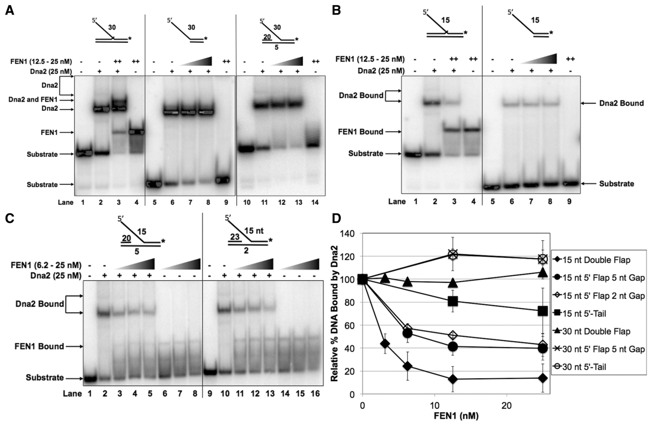
Figure 5. Binding affinity from the upstream DNA as well as a short 5' flap is necessary for Dna2 displacement by FEN1. Dna2 (25 nM) was pre-incubated with the experimental substrate prior to the addition of increasing concentrations of FEN1 (6.25, 12.5 or 25 nM as indicated in the figure headings). (A) shows Dna2 and FEN1 binding competition for the 30 nt double-flap substrate (U2:T3:D2.30), the 5'-tail substrate (T4:D2.30) and the 5 nt gap-flap (U3:T3:D2.30). (B) shows Dna2 and FEN1 binding competition for the 15 nt double-flap substrate (U2:T3:D2.15) and the 5'-tail (T4:D2.15). (C) shows Dna2 and FEN1 binding competition for the 5 nt gap-flap (U3:T3:D2.15) and 2 nt gap-flap (U4:T3:D2.15) having a 15 nt 5' flap. (D) shows the graphical quantitation of the relative percent Dna2 bound to the substrate in the absence of FEN1 or with increasing concentrations of FEN1 as defined in the 'Materials and Methods' section. In (A)–(C) the position of the Dna2–substrate complex and FEN1–substrate complex are indicated to the left and/or right of the figure. In (A), the FEN1–Dna2–substrate complex is indicated to the left of the figure. '++' represents the maximum concentration of FEN1 used.
