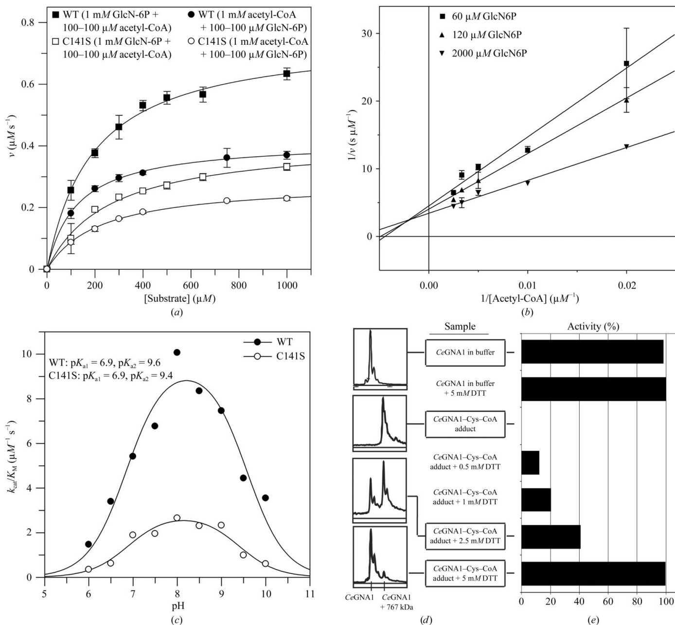
Figure 3 (a) Apparent K_m of WT and C141S CeGNA1 for both substrates. The velocity ( \mu M s^{-1} ) is shown as a function of the concentration of the second substrate. The WT enzyme has approximately twofold higher affinity for both substrates than the active-site mutant C141S CeGNA1 . The catalytic efficiency of the mutant has dropped to around 20% (Table 2). However, the covalent adduct shows no detectable signal above the background (Table 2). (b) Double-reciprocal plots of initial rates of formation of CoA catalysed by CeGNA1 . In this plot, the concentration of acetyl-CoA is varied from 50 to 500 \mu M at several fixed concentrations of GlcN-6P. (c) pH optima of WT and C141S CeGNA1 . To obtain the bell-shaped curves the nonlinear fit was calculated with GraFit . WT and C141S CeGNA1 have the same pH optimum at pH 8.2. (d) Mass spectrometry supports the covalent bond between the active-site Cys141 and the product CoA in the crystal structure (space group P6_1 ). 15 min incubation (at 293 K) with 5 mM DTT was sufficient to release the covalently bonded CoA, corresponding to the mass of one released CoA molecule (767 Da). (e) Activity of the CeGNA1 –Cys–CoA adduct dimer compared with CeGNA1 in solution after incubation with various concentrations of DTT as indicated. Incubation of 10 nM CeGNA1 –Cys–CoA without DTT does not give any detectable activity above the background. Reactivation of 98.2% can be achieved with 5 mM DTT for 15 min at 293 K.
