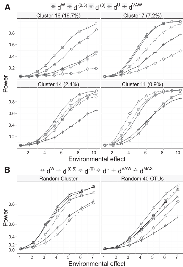
Fig. 3. Power comparison of different UniFrac variants for detecting environmental effect using tree-based simulation. PERMANOVA is used for testing hypotheses. The power curves are created by varying the degree of environmental effect. (A) The environmental factor affects a particular lineage (OTU cluster). Four example lineages of different abundance levels that are affected by environment are given. The lineage abundance is given in parentheses in the panel title. (B) The environmental factor affects a random lineage (left panel) or a random subset of 40 OTUs (right panel). The initial point of the power curve is the power when there is no environmental effect.
