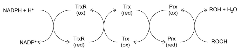
Fig. 7. Proposed electron transfer pathway of the thiol-based peroxidases: bacterioferritin comigratory protein (BCP), thiol peroxidase (Tpx), and glutathione peroxidase (Gpx). Prx in the figure is a general representation of all three thiol based peroxidases. Trx and TrxR represents thioredoxin and thioredoxin reductase, respectively.
