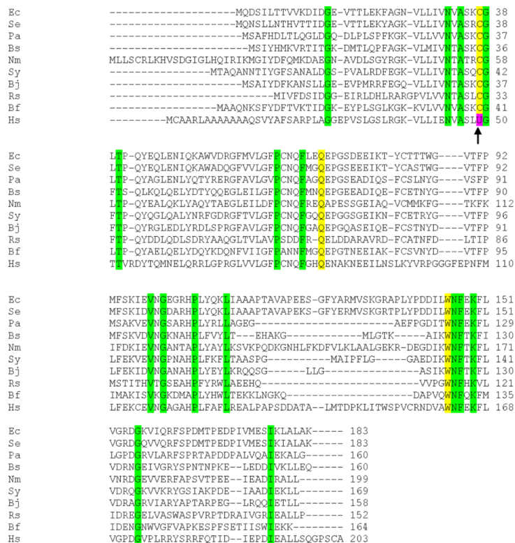
Fig. 8. Multiple sequence alignment showing conservation of glutathione peroxidase (Gpx) active-site residues (yellow) within various bacteria (Ec: E. coli ; Se: Salmonella enteric serovar Typhimurium; Pa: Pseudomonas aeruginosa ; Bs: Bacillus subtilis 168; Nm: Neisseria meningitidis ; Sy: Synechocystis sp.; Bj: Bradyrhizobium japonicum ; Rs: Rhodobacter sphaeroides ; Bf: Bacteroides fragilis ) and human glutathione peroxidase I (Hs). The presence of selenocysteine in place of cysteine in human Gpx 1 has been marked by an arrow. Other conserved residues are highlighted in green.
