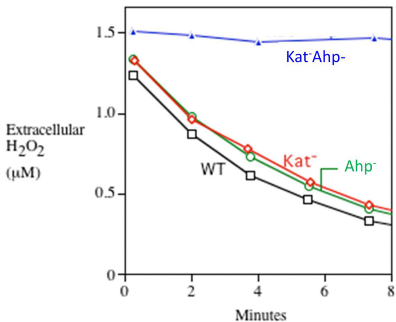
Fig. 5. H 2 O 2 decomposition by aerobic E. coli depends upon catalase and alkylhydroperoxide reductase (Ahp). H 2 O 2 (1.5 μM) was added to a dilute suspension of cells at time zero, and the amount of remaining extracellular H 2 O 2 was subsequently determined at intervals. Note that for the wild-type strain and the single mutants, the rate-limiting step in H 2 O 2 degradation was diffusion into the cell; consequently, the rates of H 2 O 2 clearance from the medium were equivalent. Measurements were made as described [10].
