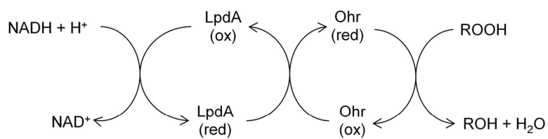
Fig. 9. Proposed electron-transfer pathway for reduction of organic hydroperoxides by organic hydroperoxide reductase (Ohr). LpdA represents the lipoylated disulfide-based enzymes that reduce oxidized Ohr.
