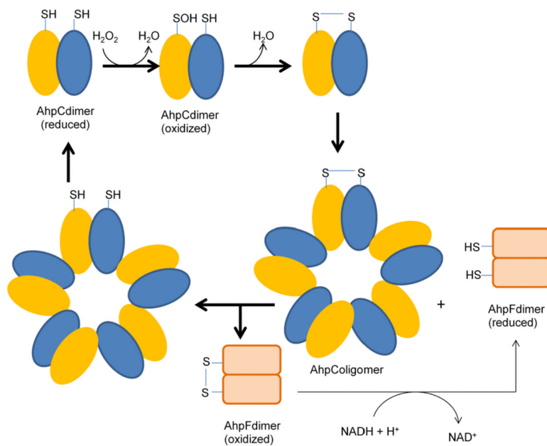
Fig. 4. The catalytic cycle of alkylhydroperoxide reductase (Ahp).
