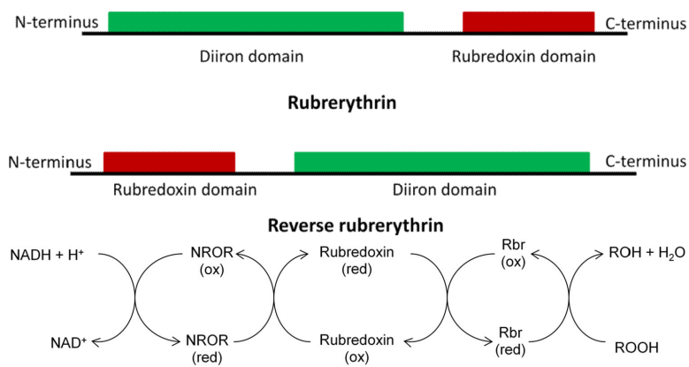
Fig. 11. Rubrerythrins. A. Domain organization. B. Scheme of electron delivery to recycle rubrerythrin (Rbr). NROR: NADH:rubredoxin oxidoreductase.
