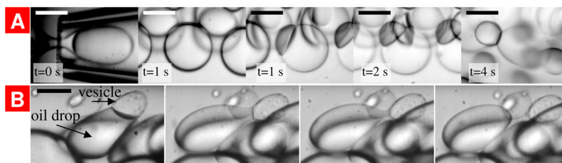
Figure 4. Microfluidic fabrication of polymersomes in a microchannel. A) Series of optical micrographs showing the generation of a double emulsion drop and the subsequent dewetting transition. Scale bars are 50 \mu\text{m} . B) Series of optical micrographs showing the separation of the polymersome from the oil drop by the shear in the microchannel. The time interval between successive images is 10 ms and the scale bar is 50 \mu\text{m} .
