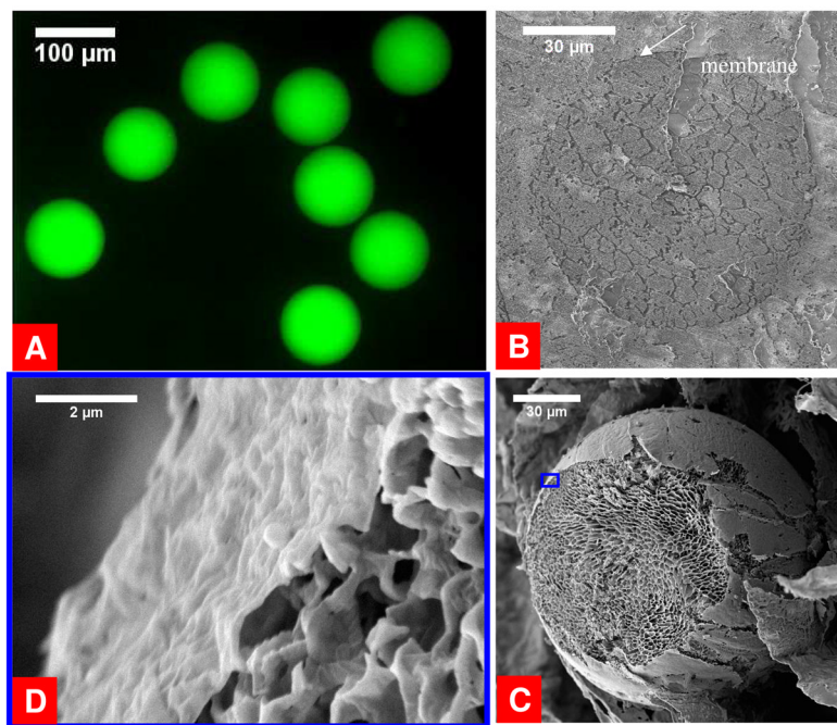
Figure 5. A) Confocal laser scanning microscope image of PEG(5000)-b-PLA(5000) polymersomes encapsulating a fluorescent dye (HPTS); B) Cryo-scanning electron microscope (Cryo-SEM) image of a PEG(5000)-b-PLA(5000) polymersome; C) Scanning electron microscope (SEM) image of a freeze-dried PEG(5000)-b-PLA(5000) encapsulating a PEG solution; D) Magnified view of the region in blue in C).
