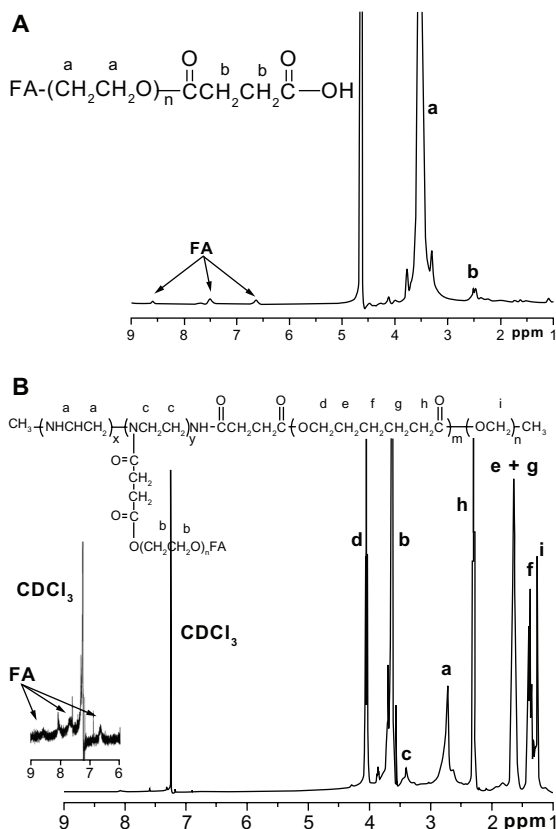
Figure 2 1 H NMR spectra (300 MHz) of (A) FA-PEG-COOH in D 2 O and (B) FA-PEG-PEI-PCL in CDCl 3 . Abbreviations: FA-PEG-COOH, folate-poly(ethylene glycol)-COOH; FA-PEG-PEI-PCL, folate-poly(ethylene glycol)-poly(ethylene imine)-poly(ε-caprolactone).
