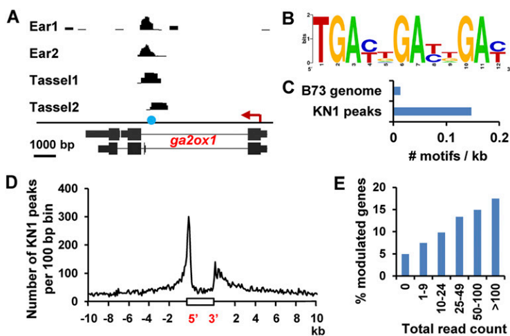
Figure 2. ChIP-seq results. (A) ChIP-seq identified KN1 binding in ga2ox1 . The blue circle indicates the position of the previously mapped KN1-binding motif, and the red arrow indicates gene orientation. (B,C) ga2ox1 -like binding motif (B) is significantly over-represented ( P -value < 1 \times 10^{-100} ) in KN1-bound loci compared with the B73 genome (C). (D) Distribution of KN1 peaks around transcribed genes. A representative gene is shown as a white box on the X-axis. (E) Relationship between the total read count and the proportion of modulated genes in all tissues.
