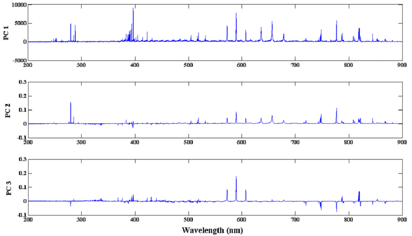
Fig. 3. The first three principal components corresponding to the entire spectral dataset acquired from the pharmaceutical samples. These three principal components, combined, explain 96.29% of the net variance in the dataset.
