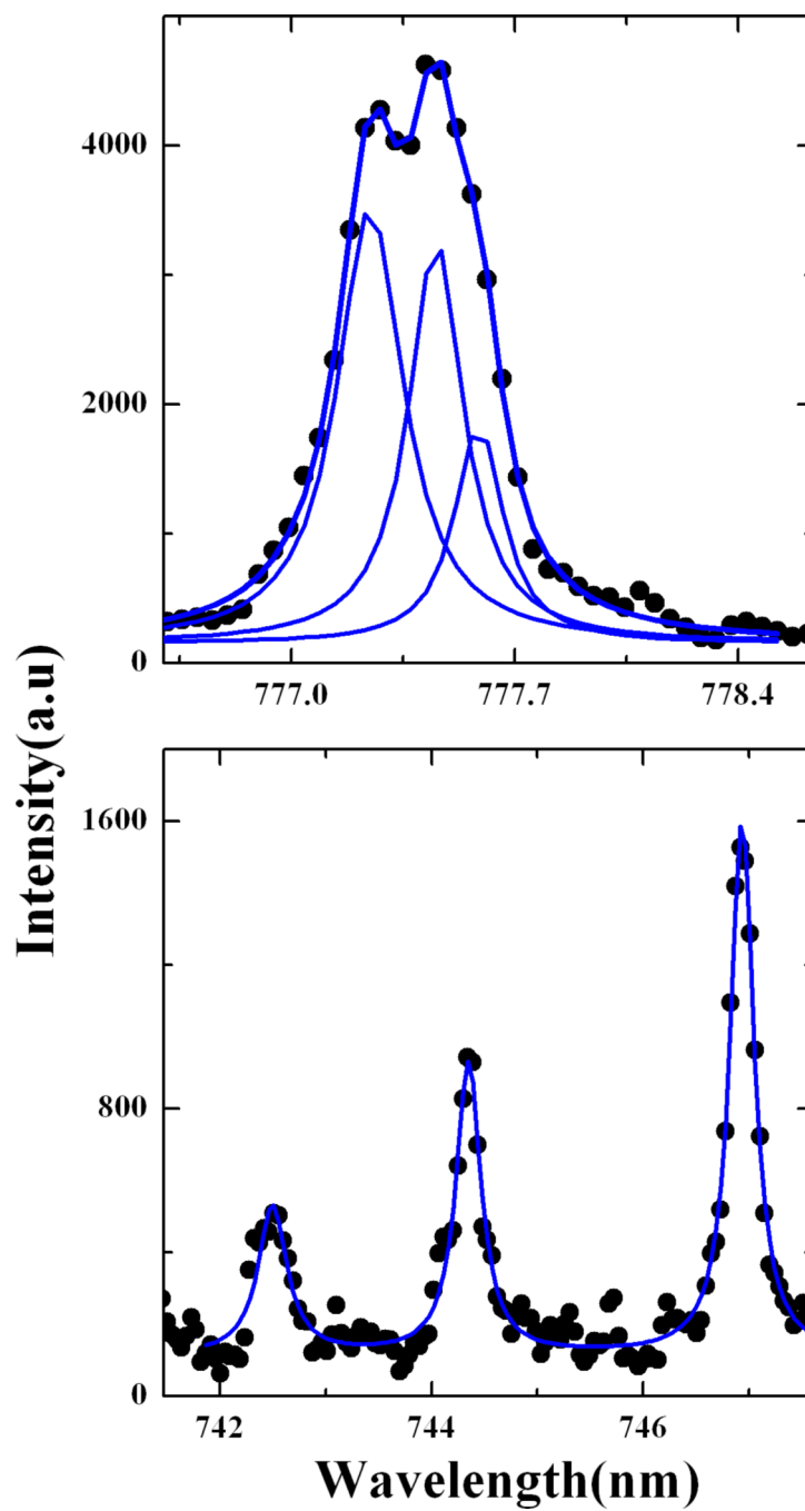
Fig. 2. a) Oxygen and b) Nitrogen LIBS peaks from the Paracetamol spectra. The dots represent the experimental points and the solid lines are the Lorentzian fits.
