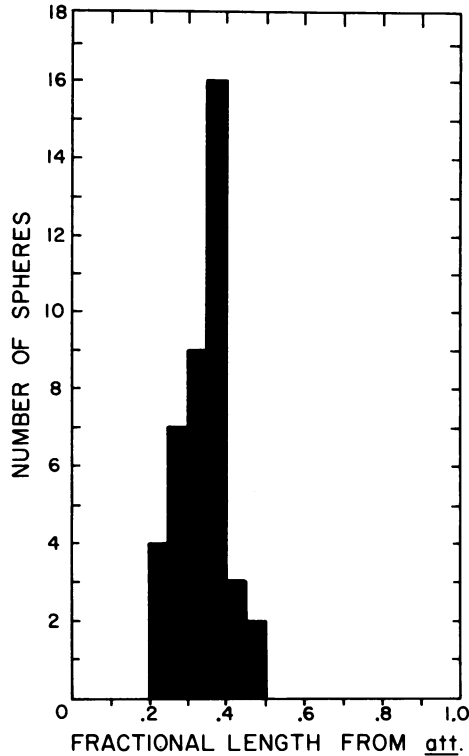
Fig. 3. Histogram of map position of tRNA tyr gene on the single strand of bacterial DNA of the \phi 80/\phi 80 psu 3 - heteroduplex. The horizontal coordinate is the fractional distance from the att site to the label. The measured position of the label is 1100 (+ 66) nucleotides from the att site.
