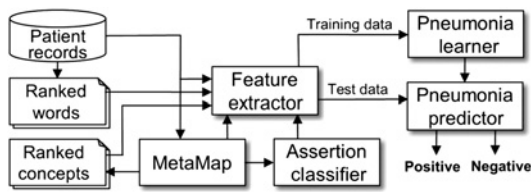
Figure 1 System architecture for pneumonia identification.
