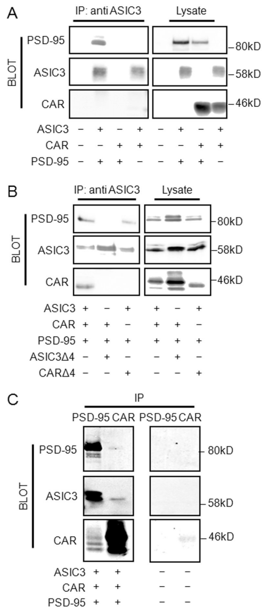
Fig. 1. CAR, ASIC3, and PSD-95 form a trimolecular complex. A) COS-7 cells were double transfected with GFP-tagged PSD-95, HA-tagged ASIC3, or FLAG-tagged CAR and subjected to IP with an antibody specific for ASIC3, followed by Western blot with tag-specific antibodies. Western blot of lysates demonstrated appropriate bands indicating successful transfection. Cells were triple transfected with GFP-PSD-95, HA-ASIC3, FLAG-CAR, HA-ASICΔ4 or FLAG-CARΔ4, and subjected to IP B) with an antibody specific for ASIC3 or C) antibodies against GFP or CAR (RmcB), followed by Western blot with GFP-, ASIC3-, or CAR (1605p)-specific antibodies. Western blot of B) lysates or C) mock transfected cells subjected to immunoprecipitation. Transfections are indicated at the bottom of each blot. Blots are representative of 3 experimental replicates.
