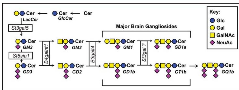
Fig. 1. Structures and biosynthetic pathways of the major brain gangliosides.
