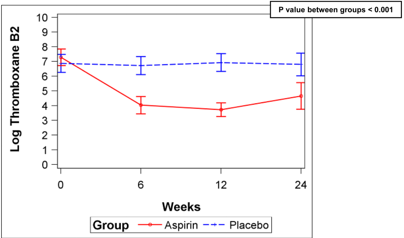
Figure 2. A) Six-minute walk distance for aspirin and placebo (error bars are 95% confidence intervals). B) Serum ln (TxB 2 ) levels for aspirin and placebo. P values from linear mixed-effects models.
