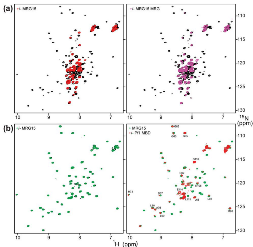
Figure 5. Pf1 PHD1 targets the MRG15 MRG domain. (a) ^1\text{H} - ^{15}\text{N} correlated spectra of ^{15}\text{N} -PHD1/MBD in the absence (black) and presence (red) of an equimolar amount of full-length MRG15 ( left panel ) and MRG15 MRG ( right panel ). (b) ^1\text{H} - ^{15}\text{N} correlated spectra of ^{15}\text{N} -PHD1 in the absence (black) and presence (green) of an equimolar amount of full-length MRG15 and in the presence of equimolar amounts of full-length MRG15 and Pf1 MBD (red). Pf1 PHD1 resonances that are relatively unperturbed upon MRG15 binding are identified. Titrations were conducted in NMR buffer comprising 20 mM Tris (pH 7.5), 50 mM NaCl, 10 \mu\text{M} \text{ZnSO}_4 , 15 mM DTT, and 0.2% \text{NaN}_3 at 25 ^\circ\text{C} . All spectra were recorded under identical solution conditions and were processed and displayed with the same parameters.
