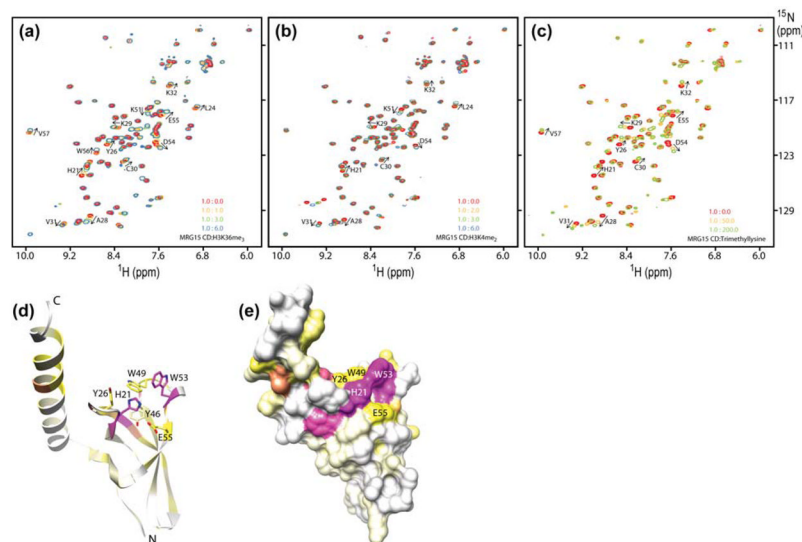
Figure 1. MRG15 chromodomain is a methyllysine binding module. Titrations of ^{15}\text{N} -labeled MRG15 CD with (a) H3K36me 3 (28–44), (b) H3K4me 2 (1–12), and (c) trimethyllysine. ^1\text{H} - ^{15}\text{N} correlated spectra of MRG15 CD were recorded as a function of increasing amounts of trimethyllysine or methyllysine-containing peptides in NMR buffer comprising 20 mM Tris- \text{d}_{11} acetate- \text{d}_4 (pH 7.5), 1 mM DTT- \text{d}_{10} and 0.2% \text{NaN}_3 at 25 °C. MRG15 CD concentrations used for the experiments in panels a-c were 0.2 mM except for panel b (0.75 mM). Chemical shift perturbations induced by H3K36me 3 (28–44) mapped on to the (d) polypeptide backbone and (e) molecular surface of the MRG15 chromodomain (PDB: 2F5K). 18 The perturbations are color ramped from white (corresponding to 0 ppm) to yellow (average + 1 standard deviation = 0.055 ppm) to magenta (average + 3 standard deviations = 0.115 ppm). Side chains of residues that form the canonical methyllysine binding pocket are shown in panel d.
