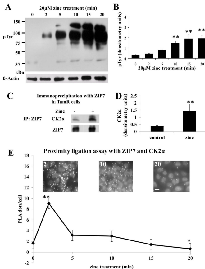
Figure 1. Zinc release activates tyrosine kinases downstream of CK2 binding ZIP7 (A-B) TamR cells were treated with 20 μM zinc plus sodium pyrithione and lysates probed by Western analysis with a phosphotyrosine (pTyr) antibody (A). pTyr, quantified by densitometry on blots from three independent experiments was normalized to β-actin and displayed as mean ± SD with significant ( P < 0.001 ) changes over time 0 indicated by ** (B). (C-D) TamR cells, treated with zinc for 5 minutes, were immunoprecipitated with antibody directed against ZIP7. Western Blot was probed with antibodies directed against CK2α (C) or ZIP7 (as loading control); mean values ± SD calculated from N=3 experiments and normalized to ZIP7 (D) showed a significant change ( P < 0.001 indicated by **) in the association of CK2α and ZIP7. (E) Proximity ligation assay was performed with anti-ZIP7 and anti-CK2α antibodies in TamR cells treated with zinc. Fluorescent dots in inserts demonstrate ZIP7 and CK2α in close proximity (<40nm). Complete time course and antibody-free controls shown in fig. S2. Pooled results as 25 stacks taken 0.3μm apart from at least 6 representative fields of view in 3 experiments are expressed as mean dots/cell ± SD. Significant changes compared to time 0 are indicated by * ( P < 0.05 ) and ** ( P < 0.001 ). Scale bar=10μm.
