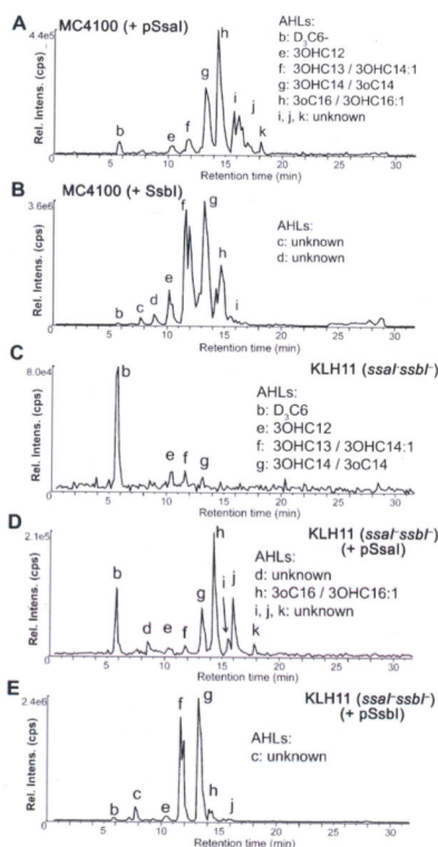
Figure 3. Mass spectrometric analysis of plasmid-expressed SsaI and SsbI-directed AHLs from E. coli and KLH11
