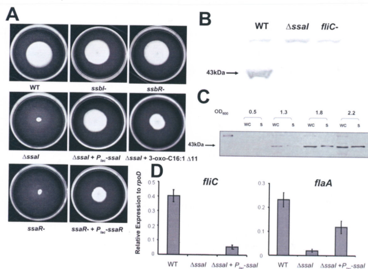
Figure 6. Regulation of swimming motility and flagellar biosynthesis by the SsaRI QS system (A) Swimming motility assays for QS mutants on 0.25% Marine Agar 2216 after 8 days at 28°C. 2 \mu M 3-oxo-C16:1 \Delta 11 was added for the \Delta ssaI mutant and pEC108 ( P_{lac} - ssaI ) and pEC112 ( P_{lac} - ssaR ) were used to complement \Delta ssaI and ssaR -mutants, respectively. (B) Antiserum raised against whole flagella from C. crescentus also recognizes KLH11 flagella. Estimated size of KLH11 flagellin is 43 kDa. (C) Flagellin synthesis during late culture stages requires ssaI . Wild type cultures were harvested at various time points along the growth curve. WC, whole culture; S, supernatant. (D) qRT-PCR results of genes fliC and flaA in wt, the ssaI deletion strain and complementation strains. Error bars are the standard deviations and results are representative of two independent experiments with triplicates.
