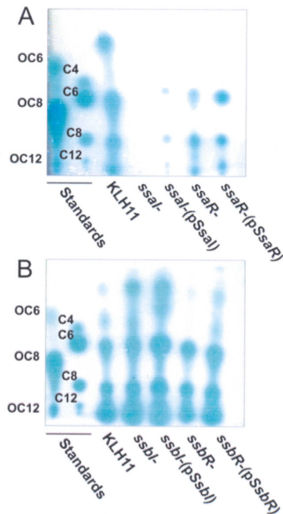
Figure 1. RP-TLC analysis of AHLs from KLH11 and quorum sensing mutants
