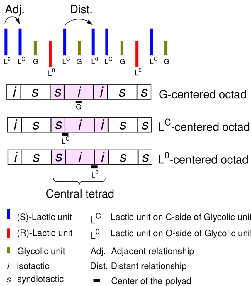
Figure 6. Example of octad-level stereosequence encoding for poly L_R L_S G L_S L_S G . The central tetrads for each type of unit are defined as including one distant and two adjacent relationships.
