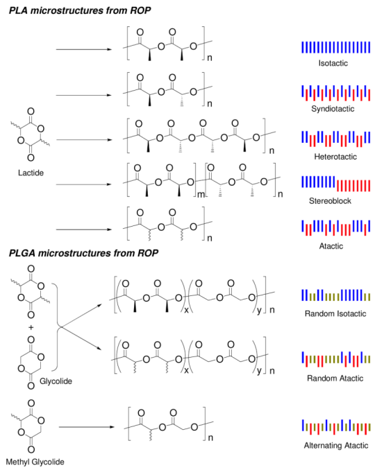
Figure 1. Comparison of complex sequences prepared by segmer assembly with simpler PLA and PLGA microstructures prepared by ring-opening polymerization. 26-31,40
