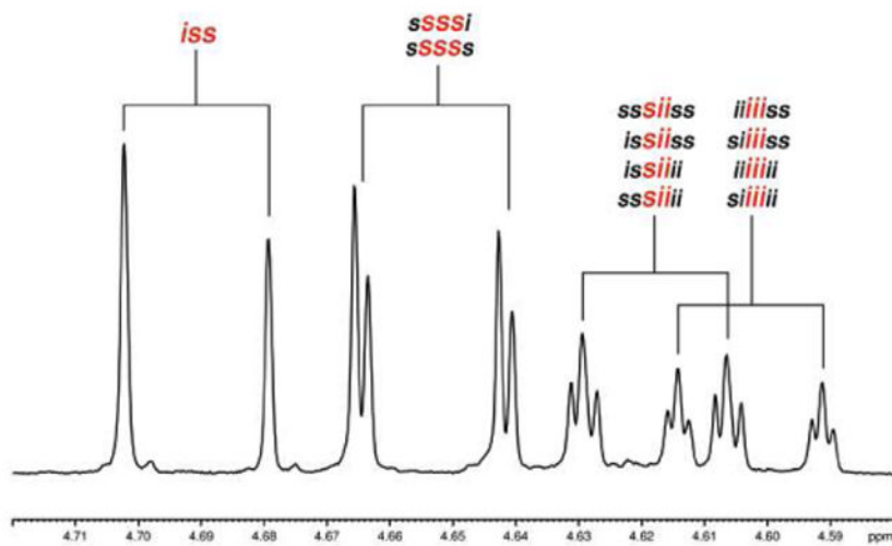
Figure 9. 1 H NMR expansion for the upfield diastereotopic proton of the glycolic methylenes of poly L rac LG (full spectrum in Figure 7). The level of sensitivity for sequence ranges from tetrad ( sii , iii ) to hexad ( sss ) to octad ( iss ) depending on the core tetrad sequence.
