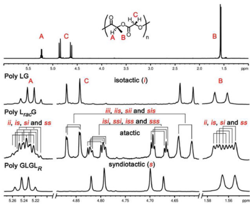
Figure 2. (Top) Full spectrum of poly LG ; (Bottom) expansions of selected regions for poly LG , L_{rac}\text{G} and \text{GLGL}_R . ^1\text{H} NMR spectra at 600 MHz in \text{CDCl}_3 .
