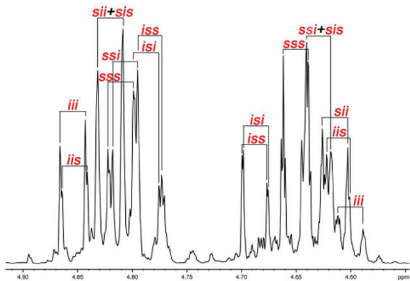
Figure 14. Glycolic methylene region of poly L rac L rac G at 700 MHz in CDCl 3 .
