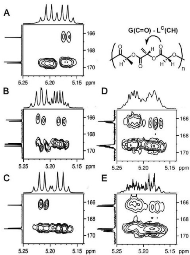
Figure 10. 2D HMBC ^1\text{H} - ^{13}\text{C} correlation NMR spectra at 700 MHz in \text{CDCl}_3 for poly LLG (A), \text{L}_R\text{L}_G\text{L}_L\text{L}_G (B), \text{L}_R\text{L}_G (C), \text{L}_{rac}\text{L}_{rac}\text{G} (D) and \text{L}_{rac}\text{L}_G (E).
