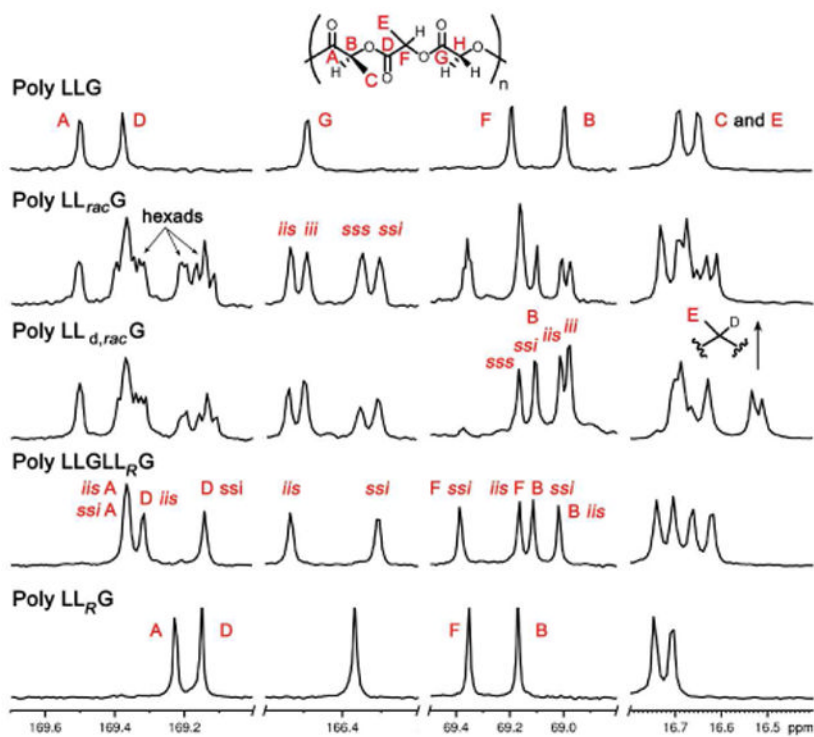
Figure 12. ^{13}\text{C} NMR spectra of LC-variable LLG polymers at 175 MHz in \text{CDCl}_3 . Comparisons of the expansions of selected regions for poly LLG , LL rac G , LL d,rac G , LLGLL R G , and LL R G .
