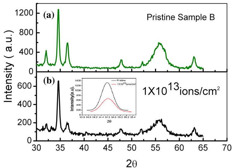
Figure 1 XRD spectra of PS-AZO nanocomposite corresponding to ZHP (PS substrate fabricated at 70 mA/cm 2 ). (a) Pristine and (b) after irradiation at a fluence of 1 \times 10^{13} ions/cm 2 . The inset shows the comparison of the (002) peak before and after irradiation.
