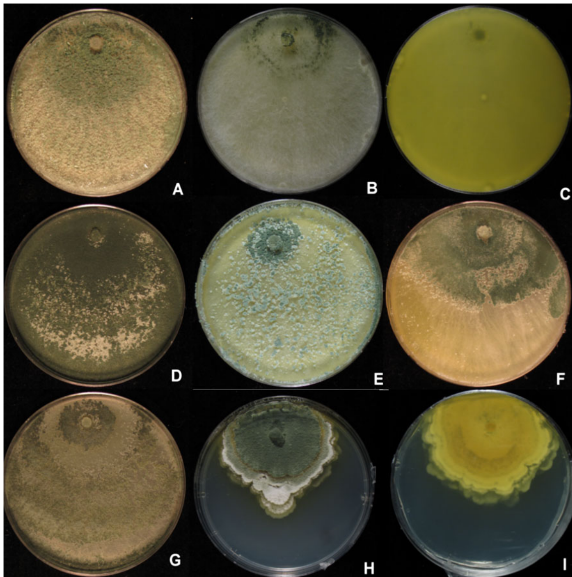
Fig. 3 Longibrachiatum Clade. Cultures grown on PDA. a–c Hypocreia orientalis ( a G.J.S. 06–317, b G.J.S. 04–321, c G.J.S. 04–316, reverse showing diffusing yellow pigment). d T. parareesei G.J.S. 04–
