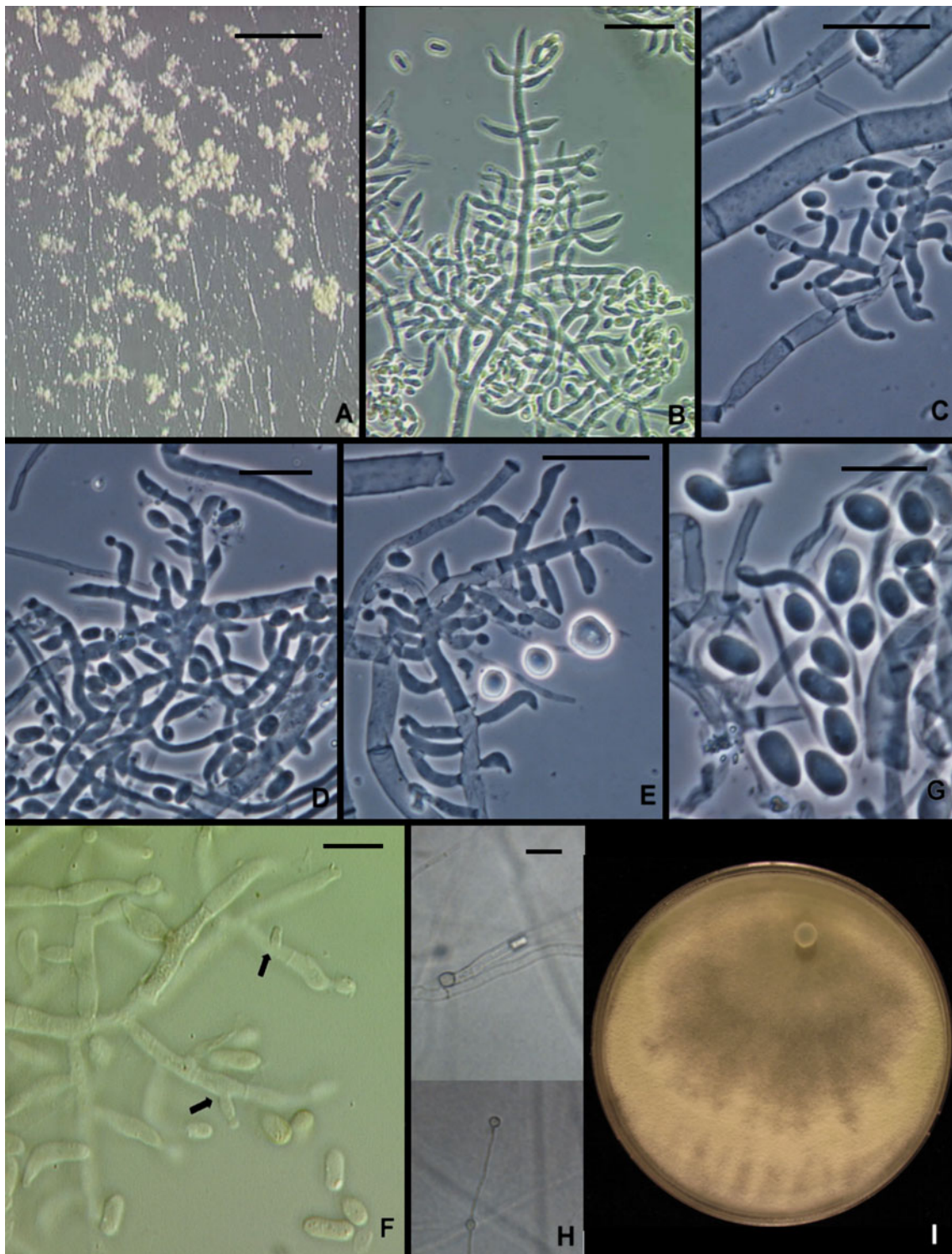
Fig. 5 Trichoderma sp. CBS 243.63. a Pustules from CMD. b–e, f Conidiophores and phialides. f, g Conidia. Intercalary phialides indicated by arrows. h Chlamydo spores. i Colony 1 week on PDA under
