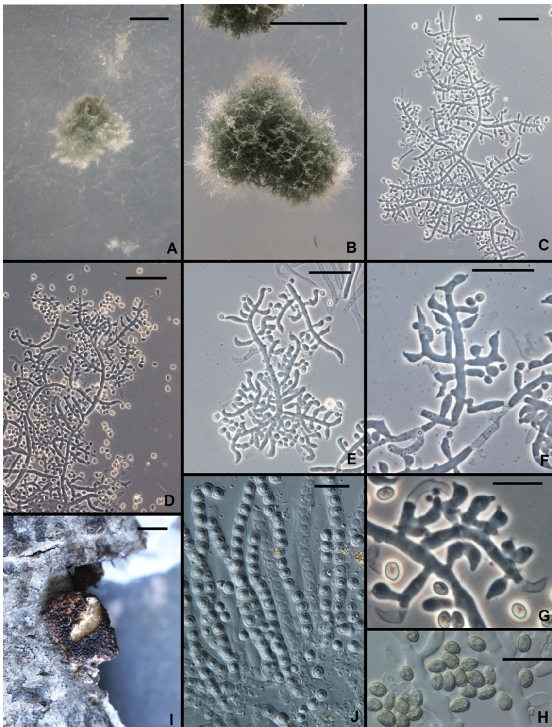
Fig. 14 Trichoderma pinnatum . a, b Pustules. c–g Conidiophores. h Conidia. i Overmature stroma. j Asci with subglobose part ascospores. a–h From SNA. a, c, e–j from G.J.S. 02–120; b, d from G.J.S. 04–100. Scale bars: a, b =0.5 mm; c–f =20 \mu m; g, h, j =10 \mu m; i =1 mm
