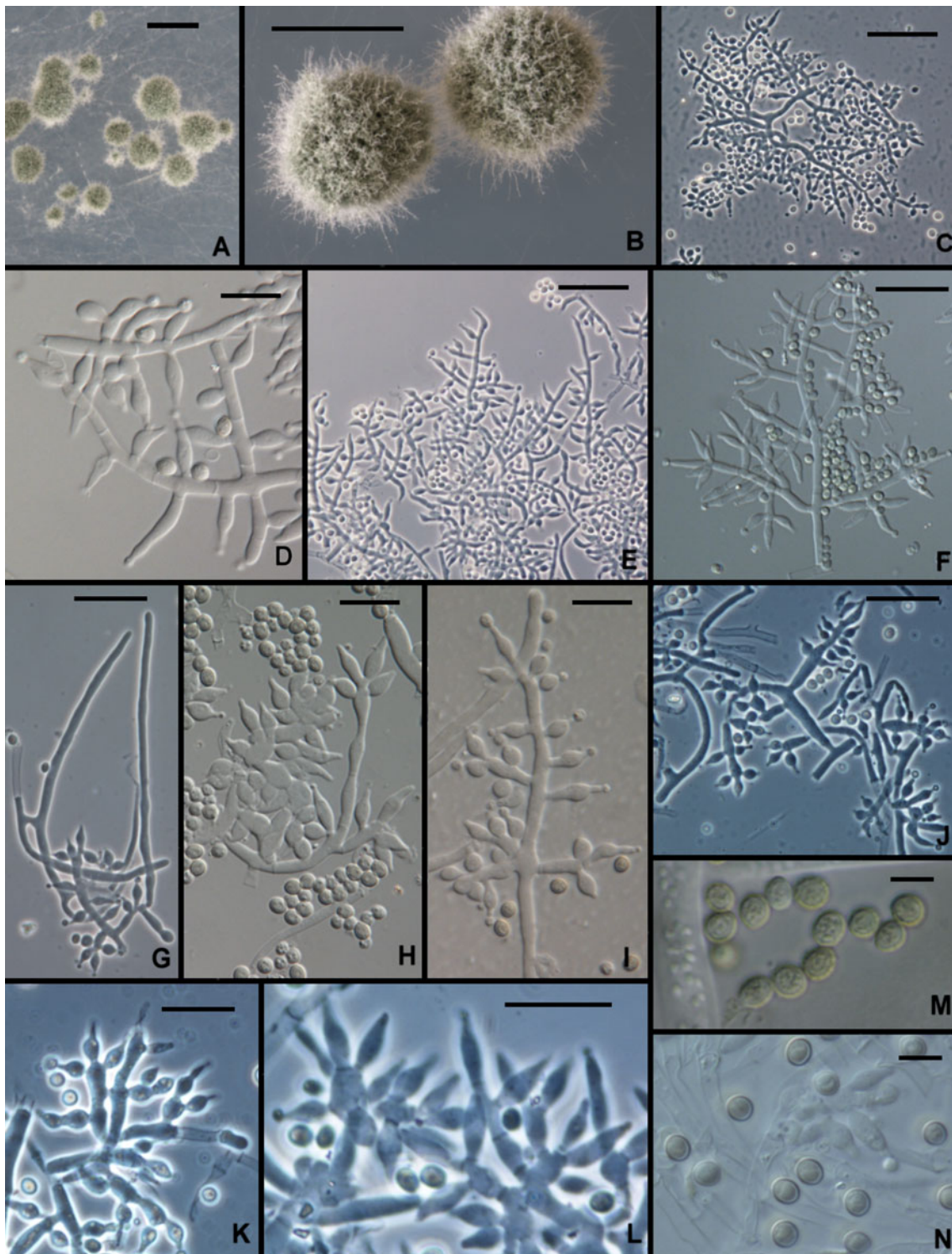
Fig. 6 Trichoderma capillare . a, b Pustules (Hairs seen in b ). c–l Conidiophores (Hairs seen in g, m ). n Conidia. All from SNA except M , which is from CMD. a–c, g–i from G.J.S. 10–170; d, e from G.J.S.
