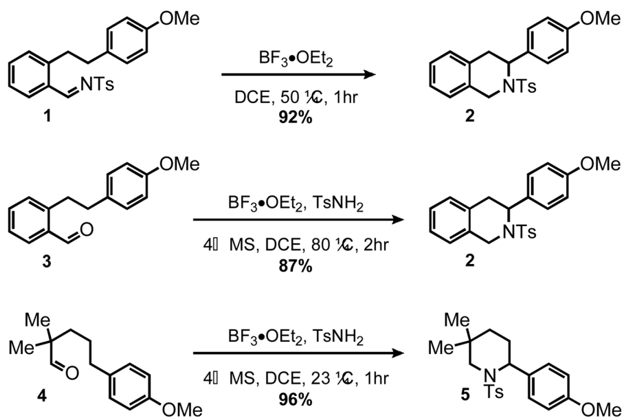
Scheme 3. One-pot Condensation/HT-amination Protocol
