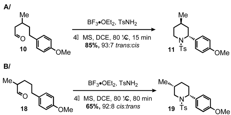
Scheme 4. HT-amination is Stereoselective
