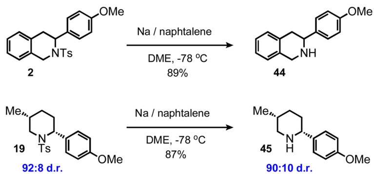
Scheme 5. Deprotection of the N -tosyl Group
