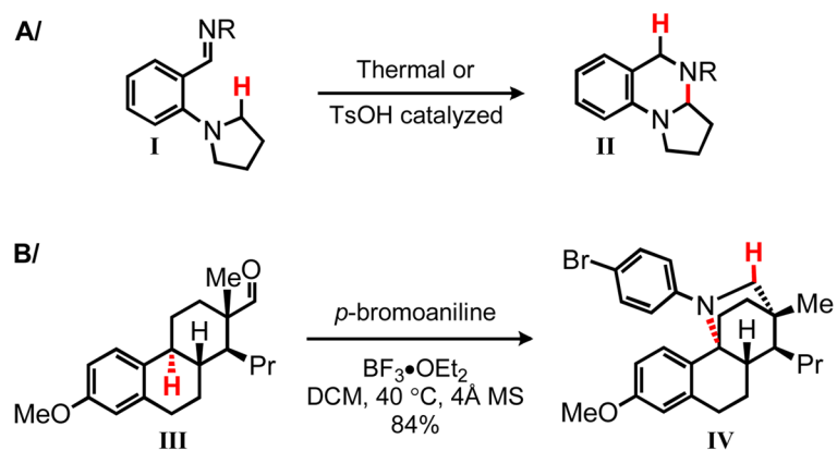
Scheme 2. Formation of Cyclic Amines via the HT-cyclization of Imines.
