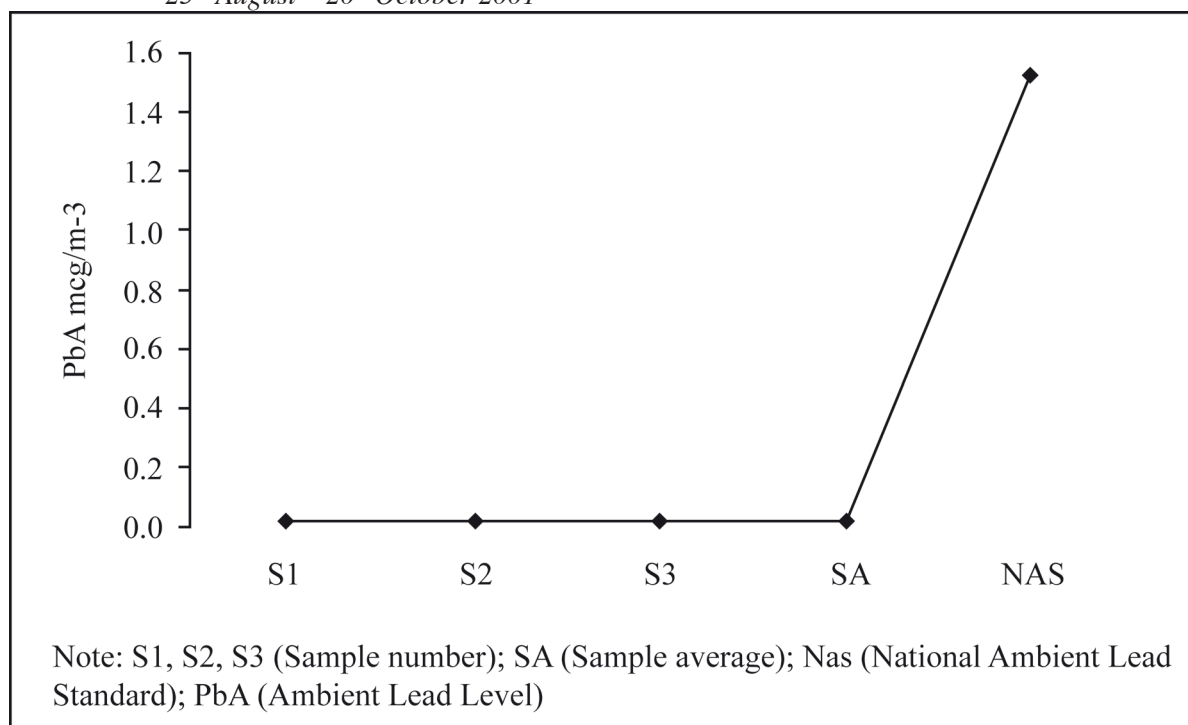
Figure 1 : Comparison of ambient lead levels measured by Continuous Air Monitoring Station at Maktab Sultan Ismail, Kota Bharu, Kelantan and the National Ambient Lead Standard, 25 th August – 20 th October 2001
