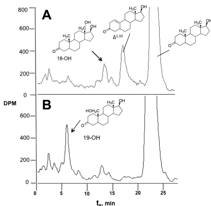
FIGURE 10. Radio-HPLC traces of [ ^3\text{H} ]dihydrotestosterone oxidation products. A, human liver microsomes; B, P450 3A4 bicistrionic membranes. The reaction time was 60 min in both cases.
