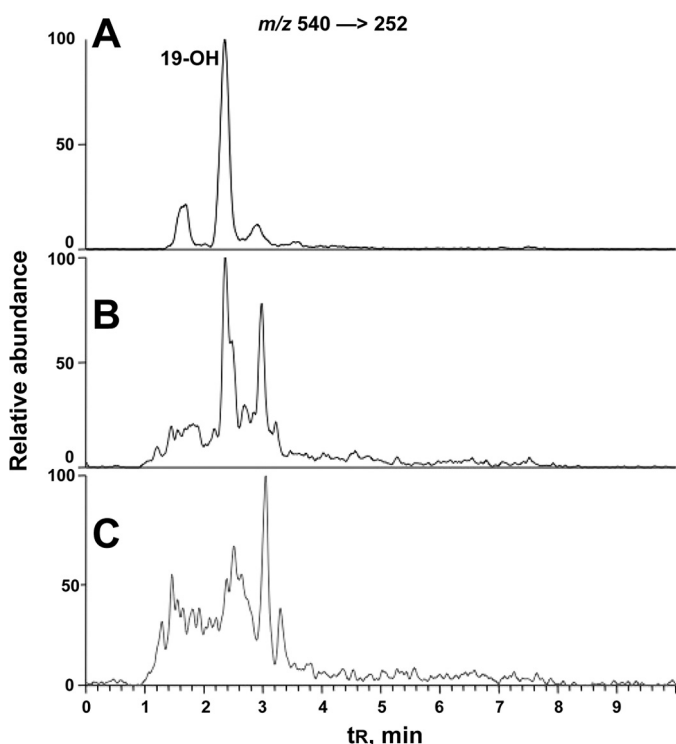
FIGURE 15. LC-MS of dansylated 19-hydroxydihydrotestosterone in human urine and plasma. The transition m/z 540 \rightarrow 252 was monitored. A, derivatization of synthetic 19-hydroxydihydrotestosterone led to one major product (identified as a mono-dansyl derivative) and two minor products (unidentified); B, dansylated 19-hydroxydihydrotestosterone in a human urine sample; C, dansylated 19-hydroxydihydrotestosterone in human plasma.
