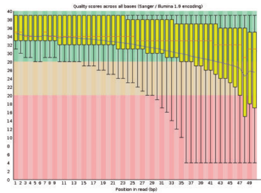
Fig. 3. Boxplots of per-base quality statistics provided by the FastQC tool (Andrews, 2010) for the MDAMB468 cell line (Sun et al. , 2011) across a random sample of the 33 million reads. The x -axis is the base position in each read, and the y -axis is the base quality score Q_b . The blue line shows the mean base quality
