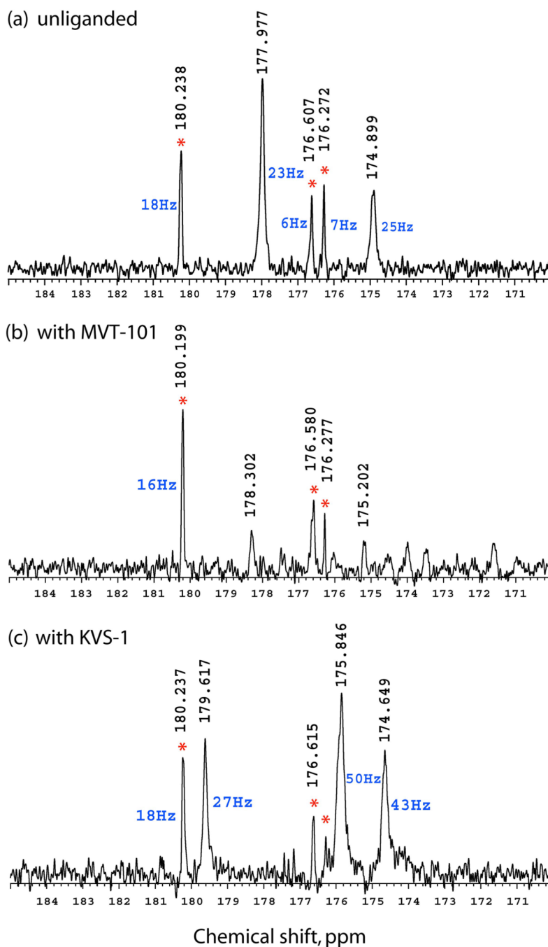
Fig. 4. 226 MHz ^{13}\text{C}\{-^1\text{H}\} NMR spectra for [L\text{-Ala}51/51']\text{HIV-1} protease: (a) unliganded; (b) complexed with the reduced isostere inhibitor MVT-101; and (c) with the ketomethylene isostere inhibitor KVS-1. Red asterisk indicates peaks originating from unfolded peptidic autoproteolysis products. [L\text{-Ala}51/51']\text{HIV-1} protease was folded by dialysis without inhibitors present; products of autoproteolysis did not exceed 5 % by HPLC-analysis. Inhibitors were added after dialysis. In (a) acquisition time was set at 0.5 s and inter-pulse delay was 1 s, while in (b) and (c) inter-pulse delay was extended to 5 s to obtain better S/N ratio spectra.
