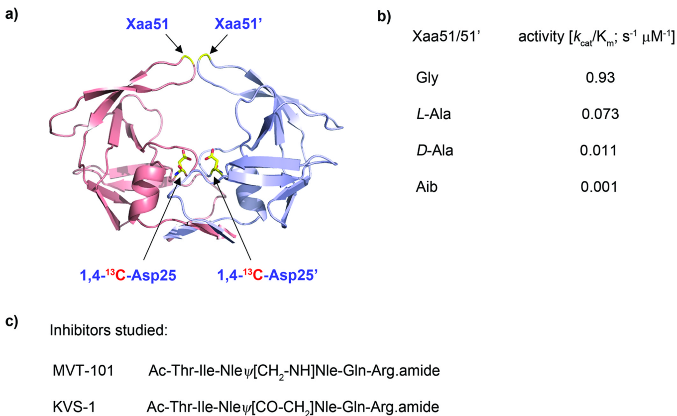
Fig. 1. (a) Catalytic dimer form ( 2 \times 99 amino acids) of HIV-1 protease. The (1,4)- 13 C-labelled Asp25/25' residues and Xaa51/51' (where Xaa = Gly, L -Ala, D -Ala, Aib) are indicated with arrows. (b) Catalytic efficiencies are listed for the wild-type HIV-1 protease (Xaa = Gly) and for three chemical analogues. (c) Inhibitors studied in this report include the reduced isostere MVT-101 and ketomethylene isostere KVS-1.
