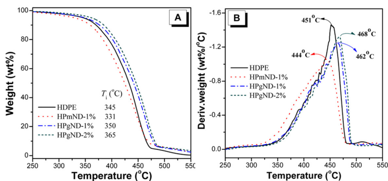
Figure 4 TGA and DTG curves of normalized weight loss rate. (A) TGA and (B) DTG curves of normalized weight loss rate by the initial sample mass at a heating rate of 20 °C/min in air condition. Notes: T_i and T_{max} were the temperatures where 5 wt.% weight loss and maximum weight loss rate occurred, respectively. T_{max} was obtained from the peak of weight loss in DTG curves.
