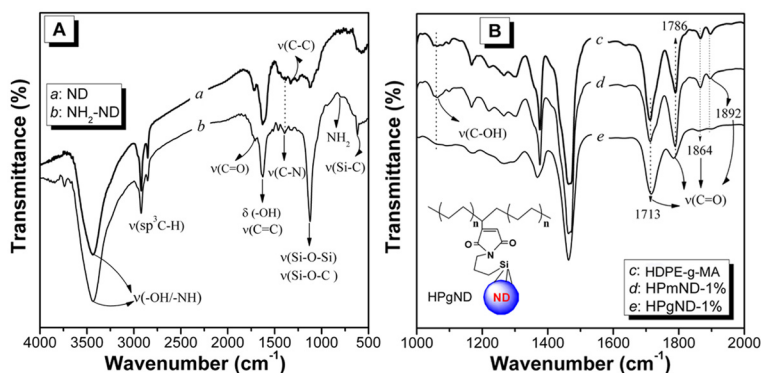
Figure 2 FT-IR spectra of pristine composites. (A) a, ND; b, NH 2 -ND; (B) c, HDPE-g-MA; d, HPmND-1.0%; and e, HPgND-1.0%.
