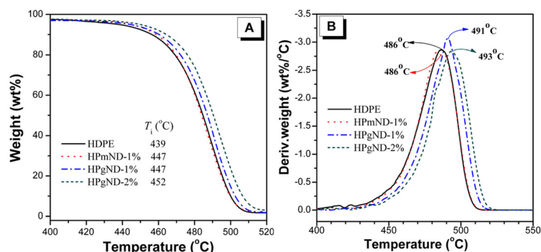
Figure 3 TGA and DTG curves of weight loss rate. (A) TGA and (B) DTG curves of weight loss rate by the initial sample mass at a heating rate of 20 °C/min in nitrogen condition. Notes: T_i and T_{max} were the temperatures where 5 wt.% weight loss and maximum weight loss rate occurred, respectively.
