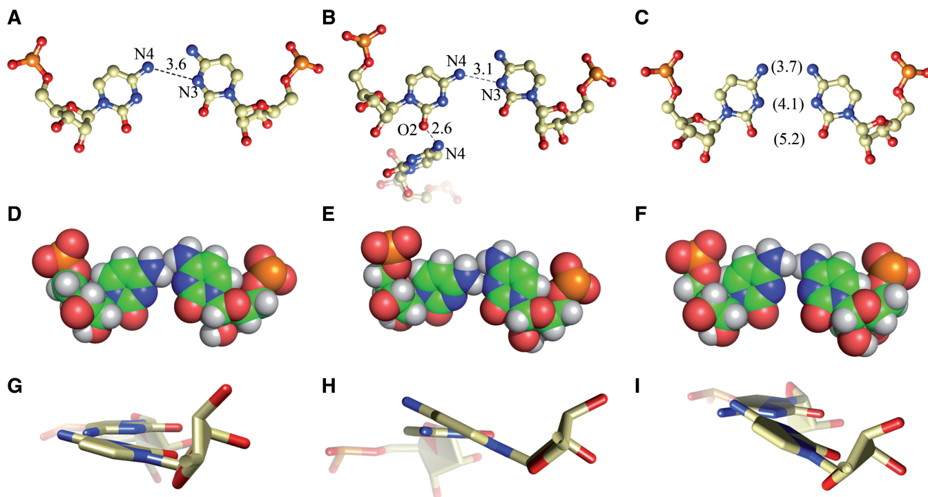
Figure 2. The three C-C pairs: from the native duplex A+B ( A , D , G ) and the LNA-containing duplexes C+D ( B , E , H ) and E+E' ( C , F , I ). The first row shows the possible H-bonds. The second row shows the Van der Waals interactions, especially the close proximity of the exo -amine groups. The third row shows the propeller twist of the bases.
