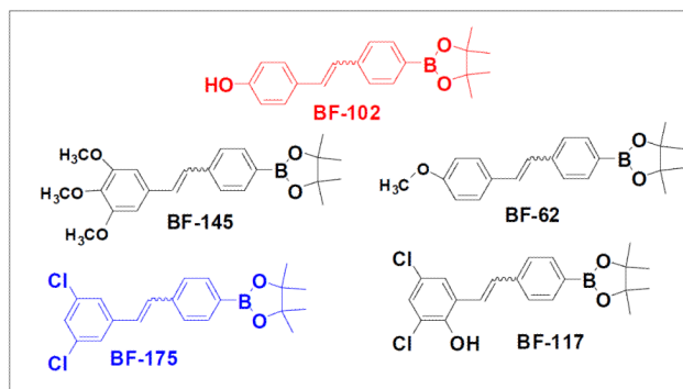
Figure 4. A small library of boron-containing compounds.
