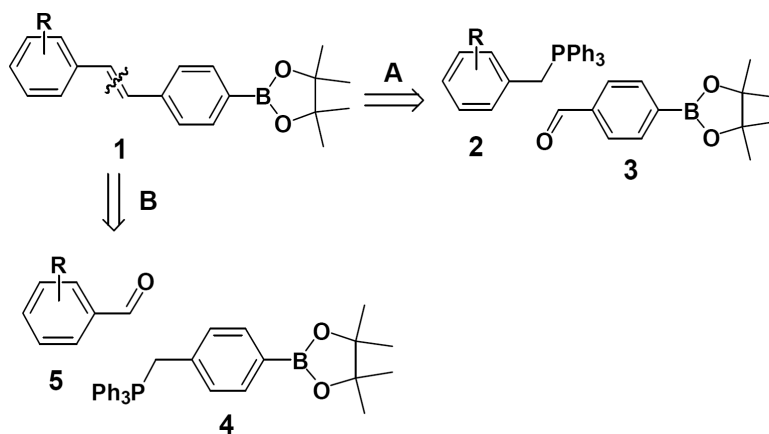
Figure 1. Retrosynthetic approach for pinacolylboronate-substituted stilbene derivatives 1 .
