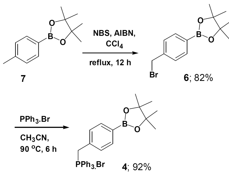
Figure 2. Synthesis of 4-(4,4,5,5-tetramethyl-1,3,2-dioxaboratophenyl)-methyl triphenylphosphonium bromide 4 .
