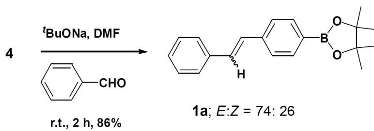
Figure 3. Proposed synthesis of stilbene 1 .
