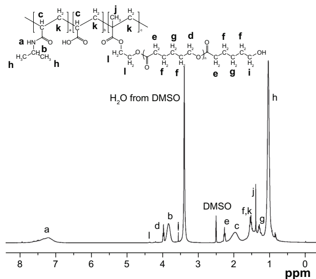
Figure 2 Proton nuclear magnetic resonance spectrum of the NIPAAm/AAc/HEMA/CL (88:9:3) copolymer.
