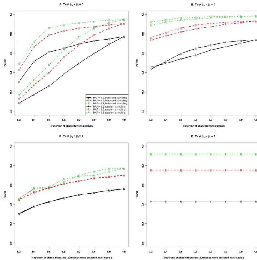
Figure 2. Power of GE-HWE under Design I when phase II subjects were selected randomly or by stratifying on E . Phase I included 1,000 cases and 1,000 controls, and the significance level was set at 0.0001. Panels A and B present the power when an equal number of cases and controls were selected into phase II. Panels C and D present the power when 300 cases were selected into phase II by stratifying on E and varying numbers of controls were selected either randomly or also by stratifying on E . Other parameters included p_e = 0.15 , e^{\beta_g} = 1.2 , e^{\beta_e} = 1.2 , and e^{\beta_I} = 1.5 .
