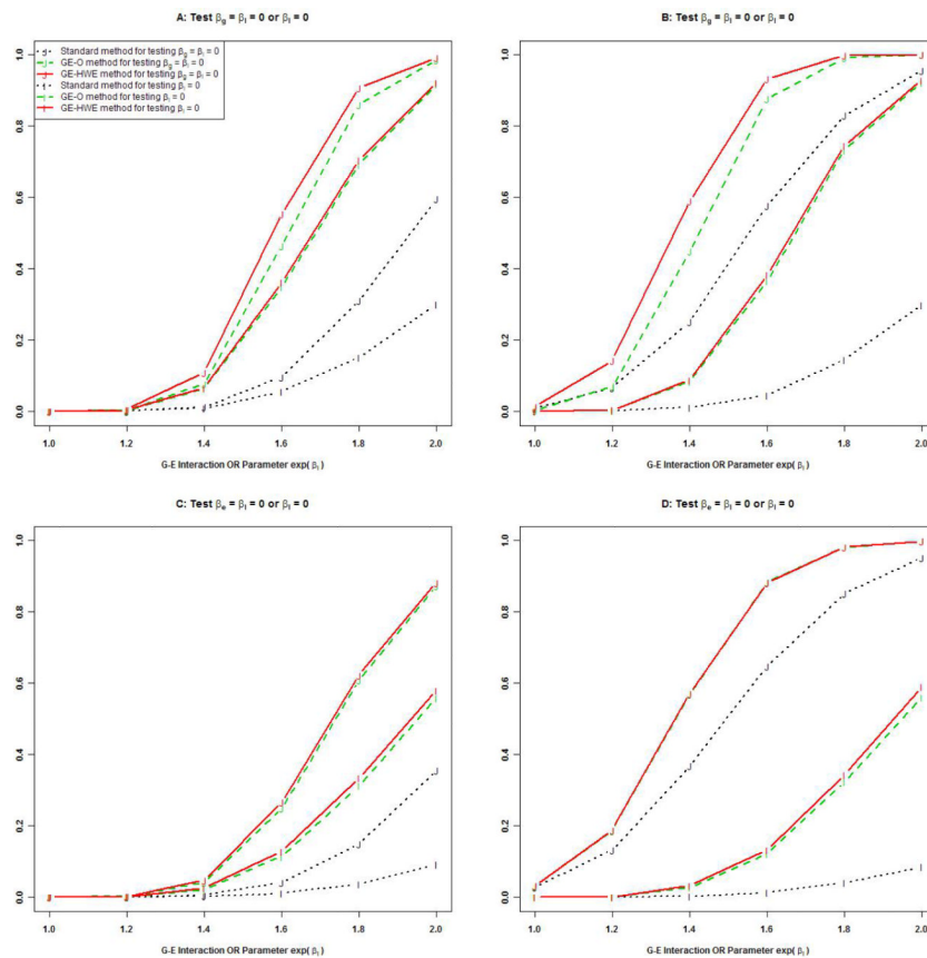
Figure 1. Power of the three methods under the standard case-control design. Panels A and B display the power for testing \beta_l = 0 or \beta_g = \beta_l = 0 in the absence (panel A) or presence (panel B) of the genetic main effect ( e^{\beta_g} = 1.2 ). Other parameters included p_e = 0.3 , p_a = 0.3 , and e^{\beta_l} = 1.5 . Each of the 1,000 replicates included 500 cases and 500 controls. Panels C and D display the power for testing \beta_l = 0 or \beta_e = \beta_l = 0 in the absence (panel C) or presence (panel D) of the environmental main effect ( e^{\beta_e} = 1.5 ). Other parameters included p_e = 0.3 , p_a = 0.3 , and e^{\beta_g} = 1.2 . Each of the 1,000 replicates included 300 cases and 300 controls. The size of the test was set at 0.0001.
