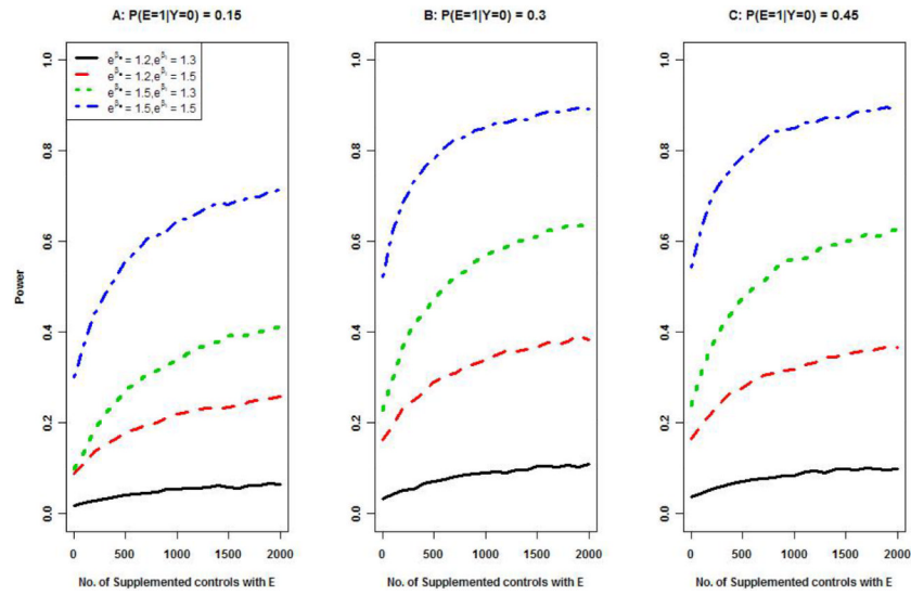
Figure 4. Power of GE-HWE for testing \beta_e = \beta_l = 0 under Supplemented Design I, where data for (G, E) for 300 cases and 300 controls was supplemented by data for E from varying numbers of controls. The significance level was set at 0.0001. The OR for the genetic main effect was e^{\beta_g} = 1.2 , and the MAF was p_a = 0.2 .
