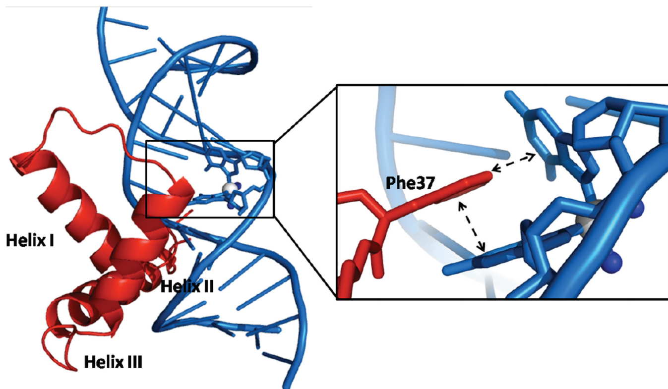
Figure 11. X-ray crystal structure of the complex of the HMGB1 domain A and a 16-bp DNA probe containing a cisplatin 1,2-intrastrand cross-link (pdb accession number 1CKD) (24). The \pi - \pi stacking and edge-to-face aromatic interactions between the side chain of Phe37 and the two platinumated guanine rings are designated by double-headed arrows.
