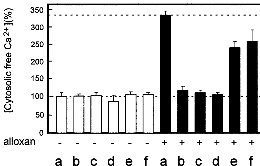
Figure 3. Effects of pretreatment with various waters on cytosolic free Ca 2+ in alloxan-treated HIT-T15 cells. After cells were pre-incubated with various waters for 24 h and treated with 1 mM alloxan for 60 min, the medium was removed, and treated with 4 \mu M Fluo 3-AM (Sigma) in HBSS buffer at 37 °C for 60 min and then washed twice. The change of cytoplasmic fluorescence intensity of selected cells was monitored by flow cytometry. The alloxan-non-treatment and alloxan-treatment were shown by – and +, respectively. Each value denotes the mean \pm S.D. of three separate experiments. a, ultrapure water (control); b, ERW; c, Hita Tenryosui water; d, Nordenau water; e, natural mineral water A; f, natural mineral water B.
