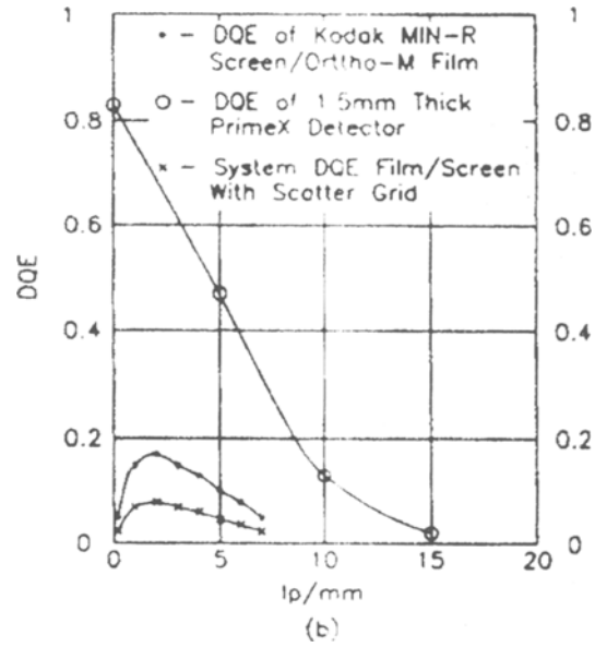
Fig 5. Primary slot scan system DQE is significantly higher than the film-screen mammography system.
