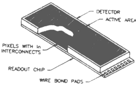
Fig 2. Hybrid radiation sensor allows for optimization and fabrication of the detector and the readout/multiplexer IC's separately.
