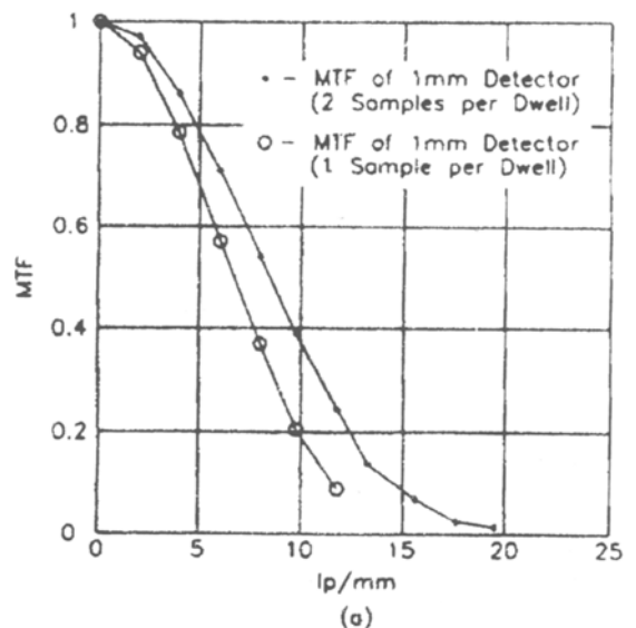
Fig 6. Measured MTF data is consistent with the predicted values.
