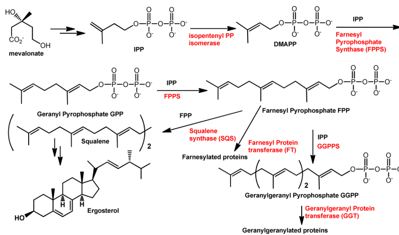
Scheme 1. Isoprenoid biosynthesis in trypanosomatids and apicomplexan parasites.
