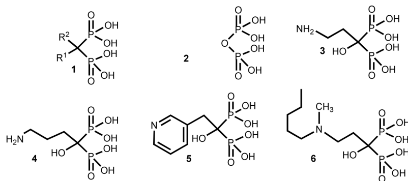
Chart 1. General formula and chemical structure of representative FDA-approved bisphosphonates clinically employed for different bone disorders.
