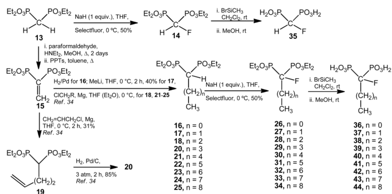
Scheme 2. Reagents and Condition for the Preparation of the Title Compounds.
