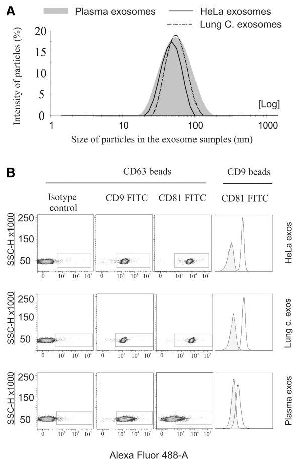
Figure 1. Characterization of exosomes. Exosomes originating from peripheral blood of healthy donors (plasma exosomes), lung cancer cells HTB-177 and HeLa cells were isolated, as described earlier (13–15). The sizes of all particles between 1 and 1000 nm in diameter present in the ultracentrifuge pellets were determined using a Zetasizer Nano (A). The presence of the exosomal surface proteins CD9, CD63 and CD81 was determined using FACS (B). For the detection of exosomal markers, the exosomes were bound to aldehyde-sulfate latex beads conjugated with anti-CD9 or anti-CD63 antibodies and analyzed by FACS.
