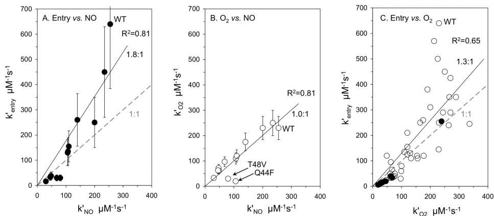
FIGURE 2. Correlation of calculated rates of ligand entry, k_{\text{NO}} , and k_{\text{O}_2} in CerHb. A , k_{\text{entry}} versus k_{\text{NO}} ; B , k_{\text{O}_2} versus k_{\text{NO}} for Val-7(B6)Ala, -Phe, and -Trp; Thr-48(E11)Val; Ala-55(E18)Val, -Leu, -Phe, and -Trp; Leu-86(G12)Ala, -Phe, and -Trp; Gln-44(E7)Trp; and Val-7(B6)Phe/Ala-55(E18)Phe/Leu-84(G12)Phe CerHb mutants (supplemental Table S2). C , k_{\text{entry}} versus k_{\text{O}_2} , open circles, all single mutants are located in and along the apolar tunnel (supplemental Table S1); closed circles, multiple mutants are located in the apolar tunnel (supplemental Table S4).
