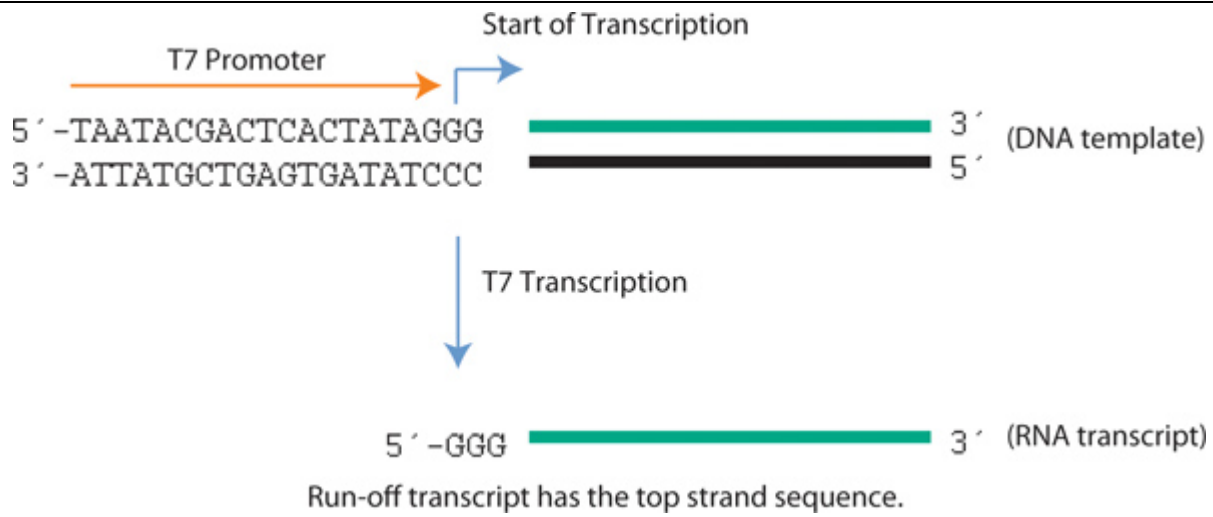
Figure 1A. RNA Synthesis by T7 RNA Polymerase
