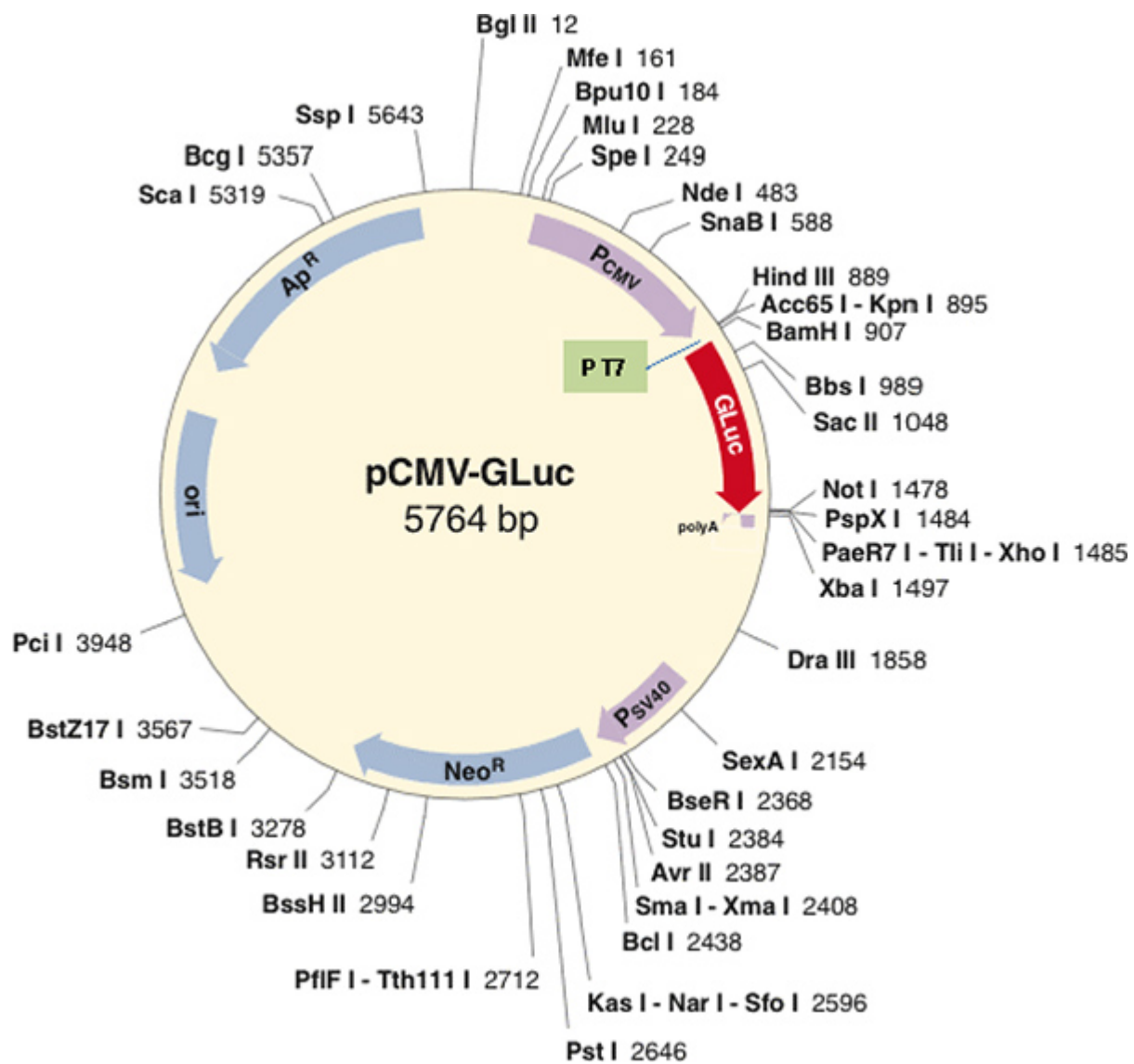
Figure 1B. pCMV-GLuc vector containing GLuc gene and T7 promoter.
