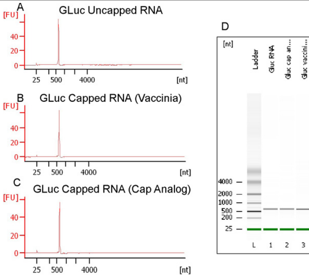
Figure 2. Bioanalyzer electropherograms and gel- image of capped and uncapped RNA . The X-axis is the size of the RNA in nucleotides (nt) and the Y-axis represents fluorescence units (FU). A) Electropherogram of GLuc mRNA (uncapped) after purification. B) Electropherogram of GLuc mRNA (capped using Vaccinia capping enzyme). C) Electropherogram of GLuc mRNA (capped co-transcriptionally using cap analog). D) Gel-like image generated by the Bioanalyzer. The 'L' lane is the RNA ladder, Lane 1 is uncapped GLuc mRNA, Lane 2 is GLuc mRNA capped using the cap analog and Lane 3 is the GLuc RNA capped using Vaccinia capping enzyme.
