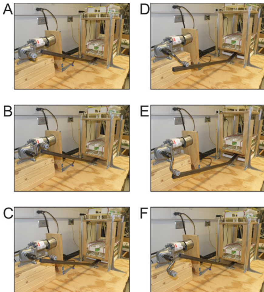
Figure 1. Operation of the Power Tower. (A-C) The motorized bent arm with attached roller rotates clockwise until it comes into contact with the bent square tube. (D,E) The arm pushes down on the bent square tube, causing the platform that is laden with vials of flies to lift. (F) As the arm clears the tube the platform is allowed to fall back down, forcing the flies to return to the bottom of the vial.
