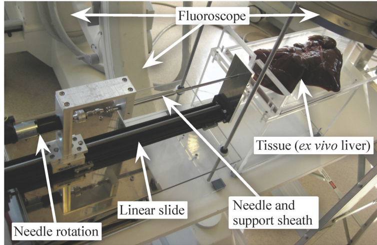
Fig. 7. Our portable needle steering device is designed to fit under a fluoroscope while allowing control of the needle's insertion and rotation. When using conventional fluoroscopy, only one image plane is available, so the planar controller is unable to determine the height of the needle. Our experimental validation used a similar device that uses two cameras to triangulate the needle tip inside a transparent artificial tissue. Clinical procedures will use bi-plane fluoroscopy or 3D ultrasound to directly measure the needle tip position inside the tissue.
