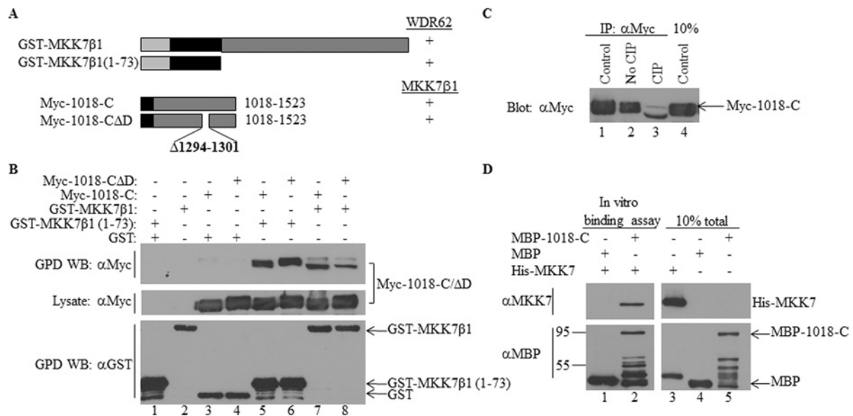
Figure 8 MKK7 \beta 1 N-terminal extension associates directly with WDR62 independently of JNK
