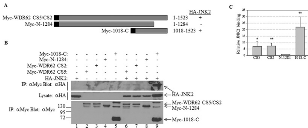
Figure 2 WDR62 C-terminal domain is necessary for JNK association
