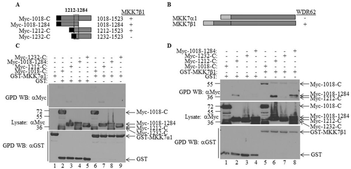
Figure 7 WDR62 associates with MKK7 \beta 1, but not with MKK7 \alpha 1
