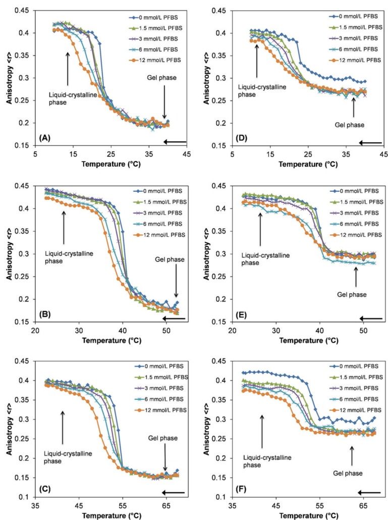
Figure 2. Fluorescence anisotropy as a function of temperature for PC – PFBS mixtures. Representative plots from at least three experiments are shown. The liquid-crystalline and gel phases are indicated by arrows. DPH was used as the probe for (A) DMPC – PFBS, (B) DPPC – PFBS and (C) DSPC – PFBS. TMA-DPH was used as the probe for (D) DMPC – PFBS, (E) DPPC – PFBS and (F) DSPC – PFBS. The samples were cooled at a rate of 0.2 °C/min, as indicated by the arrows.
