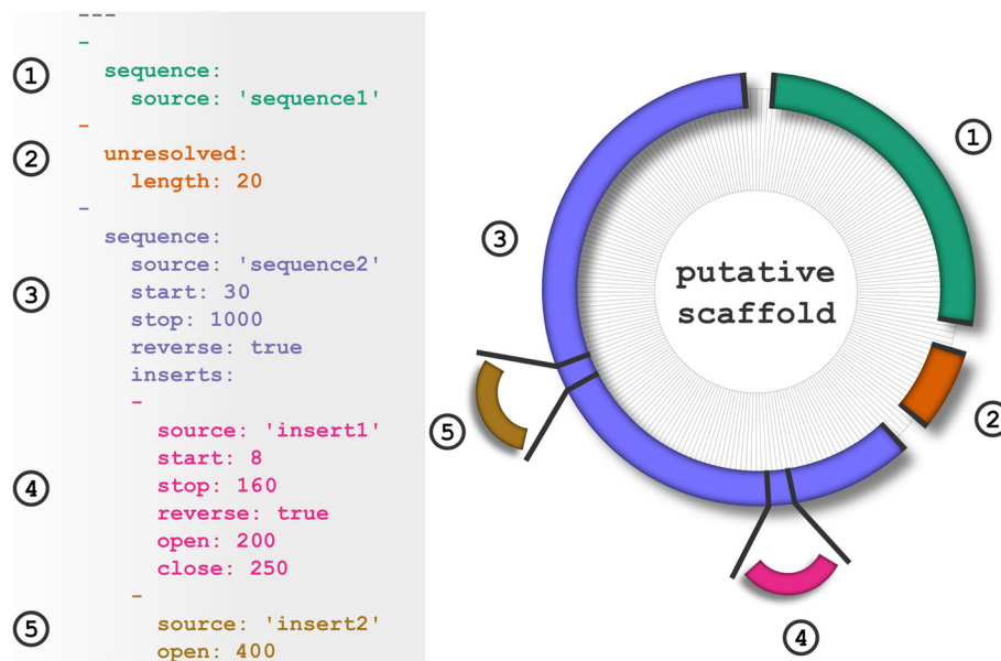
Figure 1 Example of Scaffolder File and the Resulting Build An example scaffold file written using the YAML syntax [1] (left) and the resulting putative scaffold sequence (right). The scaffold contains three entries and two inserts. Each entry in the scaffold file text is delimited by a '-' on a new line and highlighted using separate colours. The scaffold diagram on the right is not to scale and instead illustrates how the scaffold sequences are joined.
