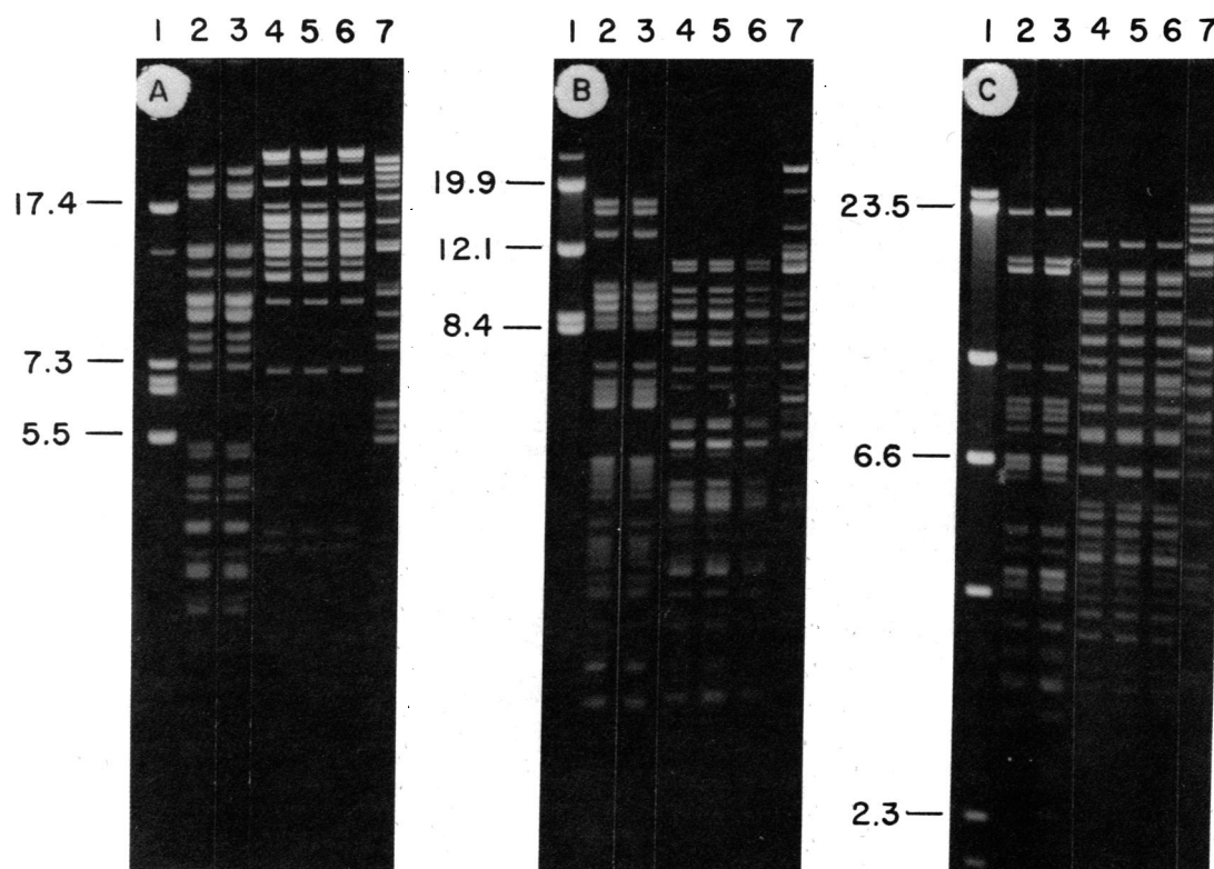
FIG. 2. Electrophoresis of algal virus DNAs after treatment with Bam HI (A), Sma I (B), and Hind III (C). The DNAs used were \lambda DNA (lane 1) and viral DNAs isolated from Chlorella -like algae from Florida (lane 2), Wards (lane 3), Carolina (lane 4), Sargent-Welch (lane 5), and Nebraska (lane 6) hydra and from paramecia (lane 7). Sizes of some of the \lambda fragments (kilobase pairs) are given.
